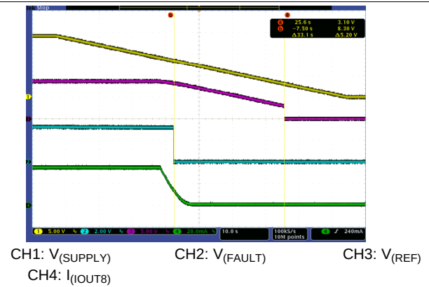
Figure 26. Slow Power Down ( V_{(SUPPLY)} , V_{(EN)} , V_{(PWMx)} Fall Together From 14 V to 0 V by 0.2 V/s)
