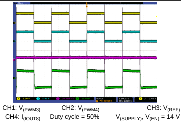
Figure 27. PWM Dimming, Dimming Frequency = 1000 Hz
