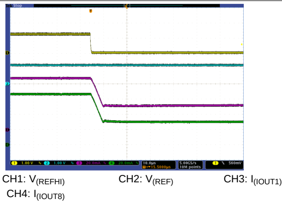
Figure 29. Load Transient, I_{(OUTx)} Decreases From 70 mA to 35 mA
