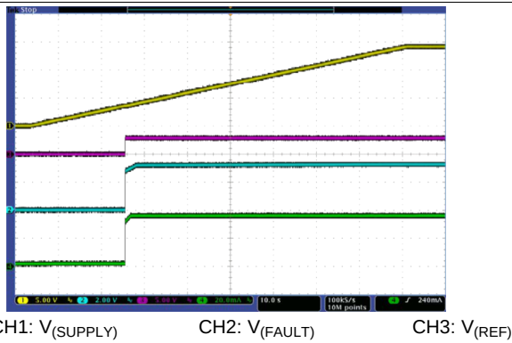
Figure 25. Slow Power Up ( V_{(SUPPLY)} , V_{(EN)} , V_{(PWMx)} Rise Together From 0 V to 14 V by 0.2 V/s)
