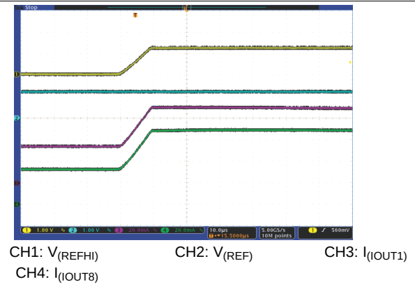
Figure 28. Load Transient, I_{(OUTx)} Increases From 35 mA to 70 mA
