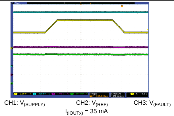
Figure 30. Line Transient, V_{(SUPPLY)} , V_{(EN)} , V_{(PWMx)} Ramp From 9 V to 16 V to 9 V by 0.1 V/μs
