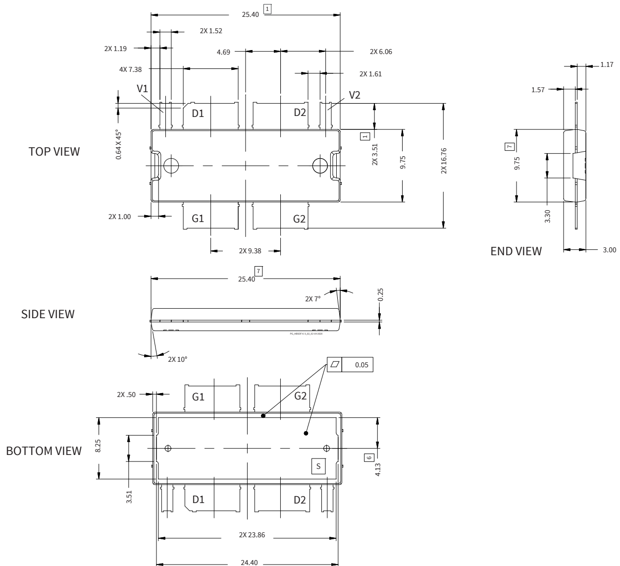
Package PG-HBSOF-6-3
