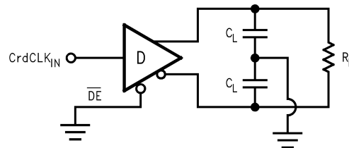
Figure 6. Driver Propagation Delay Test Circuit
