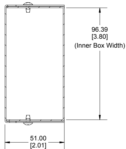
SECTION A-A End View of Assembly
