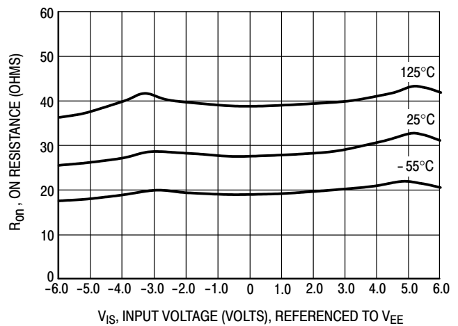
Figure 10. Typical On Resistance, V_{CC} - V_{EE} = 12.0 \text{ V}
