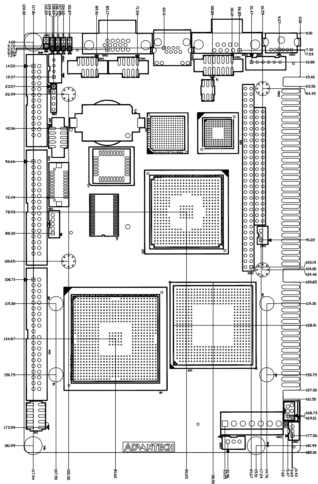
Figure 1.1 Board Layout: Dimensions (Component Side)
