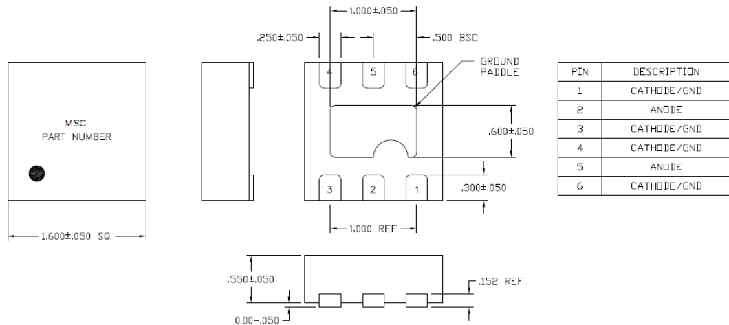
Figure 20 • Package Dimensions
