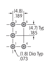
Maximum Panel Thickness .197" (5.0mm)
