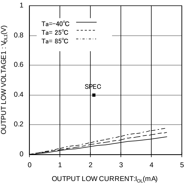
Figure 6. Output Low Voltage1 vs Output Low Current ( V_{CC}=2.7\text{V} )
