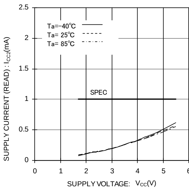
Figure 17. Supply Current (READ) vs Supply Voltage (f SK =3MHz)
