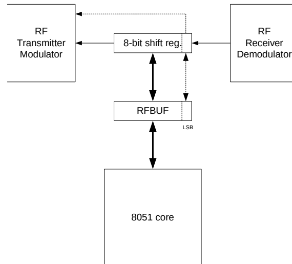
Figure 24. RF Data Buffering. Dotted lines show bitmode
