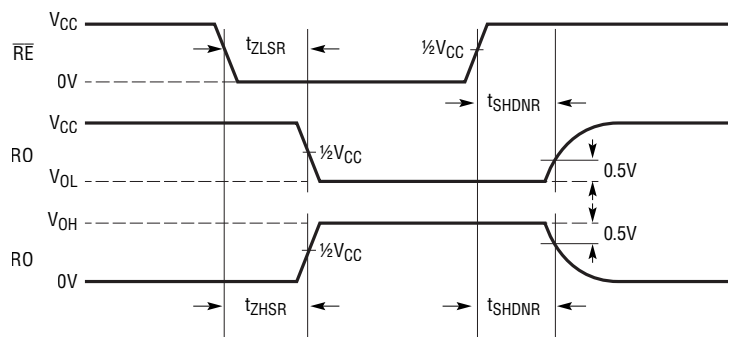
Figure 9. Receiver Shutdown Timing Measurements
