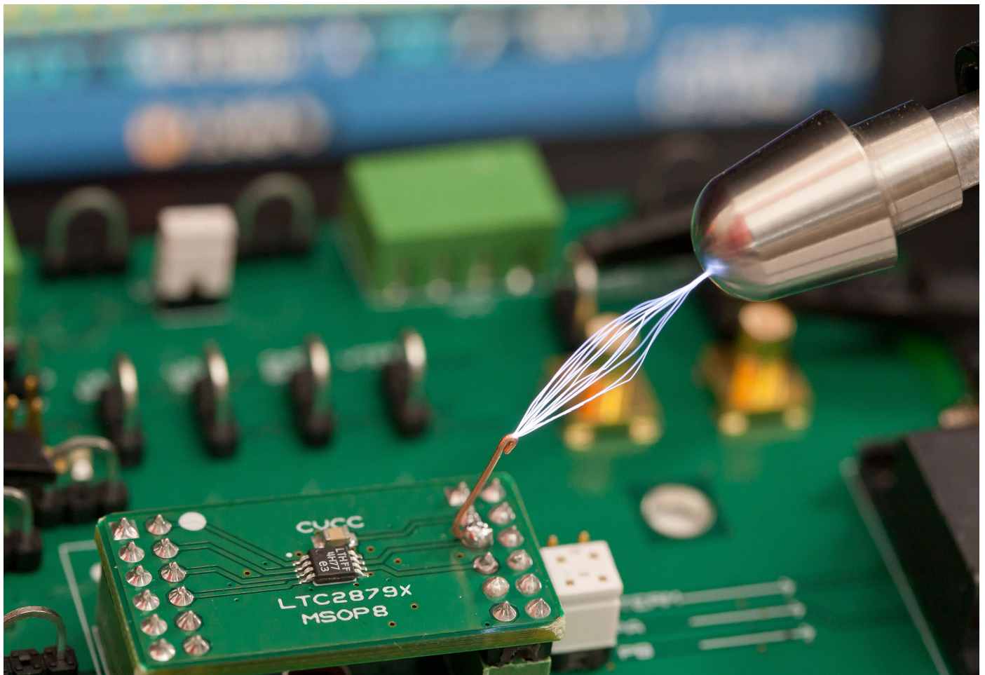
Figure 14. This Single Exposure Image Captures the Striking Robustness of an Unprotected LTC2879X Hit Repeatedly with 26kV ESD Discharges While Operating without Damage or Circuit Latchup
