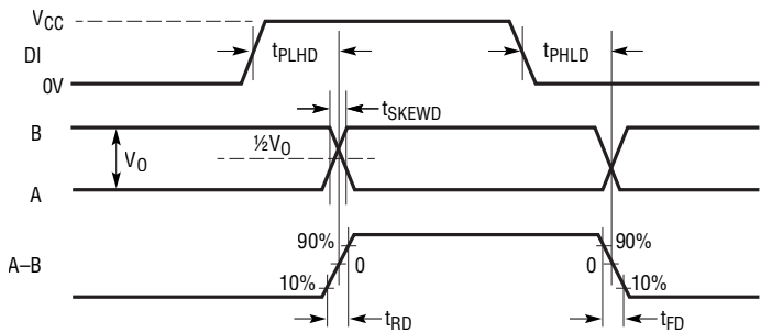
Figure 5. Driver Timing Measurement
