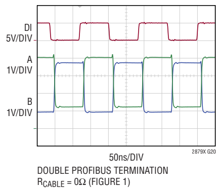
PROFIBUS Operation at 12Mbps V_{CC} = 5\text{V}
