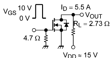
Duty \leq 1\% , t_w = 10\text{ }\mu\text{s} Fig. 6.2.1 Switching Time Test Circuit
