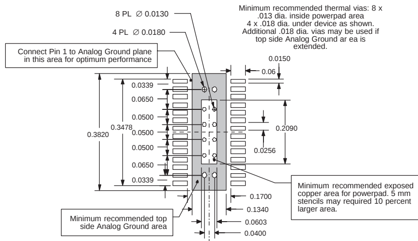
Figure 9. Recommended Land Pattern for 28-Pin PWP PowerPAD
