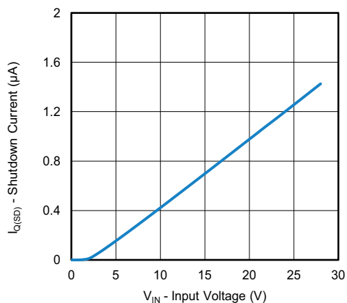
Fig. 6 - Shutdown Current vs. Input
