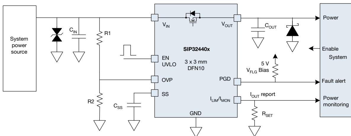
Fig. 1 - Application Circuit
