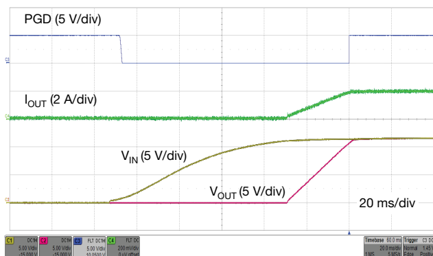
Fig. 23 - Turn On by V_{IN} V_{IN} = 12\text{ V} , R_L = 6\ \Omega , C_L = 220\ \mu\text{F} , C_{SS} = 133\text{ nF} , R_{LIM} = 1.74\text{ k}\Omega EN Voltage Divider Resistors, 1 M \Omega and 127 k \Omega
