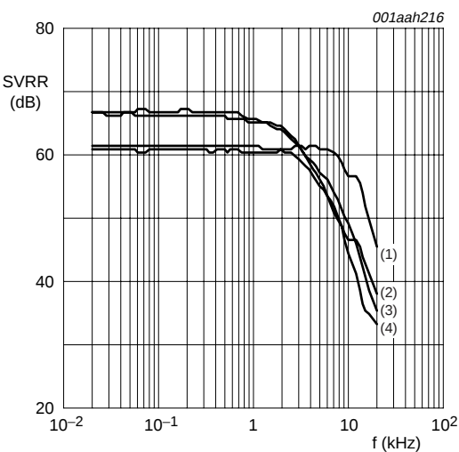
Fig 24. Supply voltage ripple rejection as a function of frequency; Mute mode
