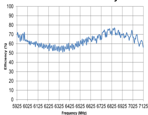
6 / 7 GHz Efficiency
