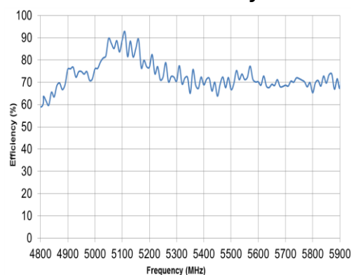
5 GHz Efficiency
