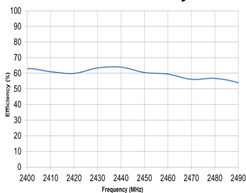
2.4 GHz Efficiency
