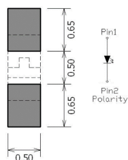
Figure 1. IN-S42CTQIR Solder Pattern
