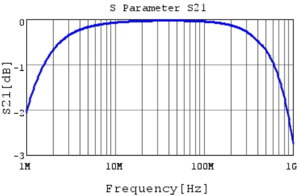
DE1E3RA222MJ4BN01F S21 DCOV, 20degC
