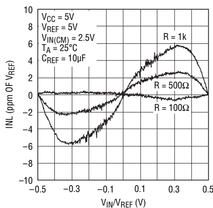
Figure 15. INL vs Differential Input Voltage and Reference Source Resistance for C_{REF} > 1\mu F
