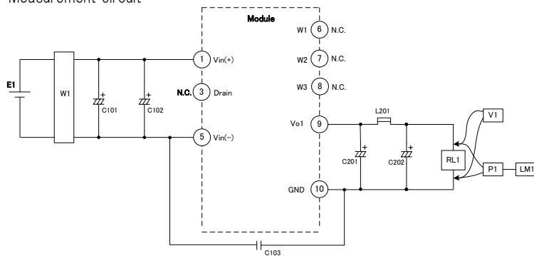
Measurement circuit
