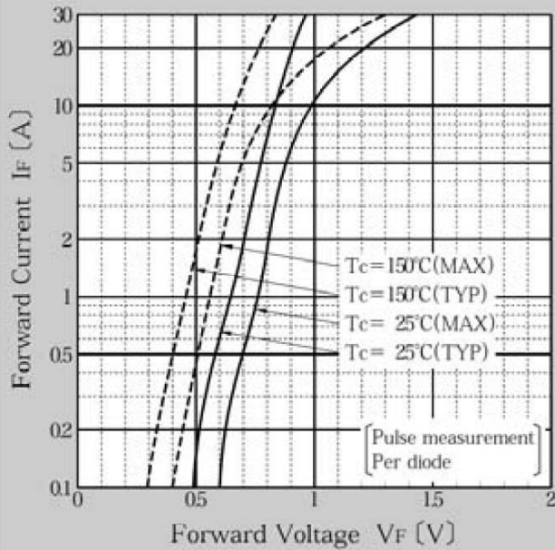
Forward Voltage
