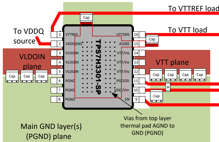
Figure 9-1. Layout Recommendation
