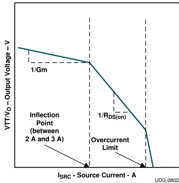
Figure 8-9. TPS7H3301-SP Impedance Characteristics
