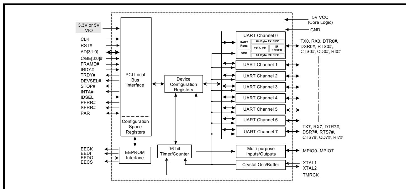
FIGURE 1. BLOCK DIAGRAM
