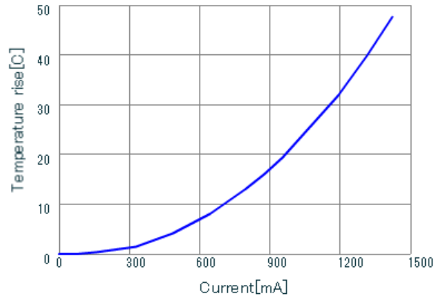
LQH44PN100MJ0 DT_Current
