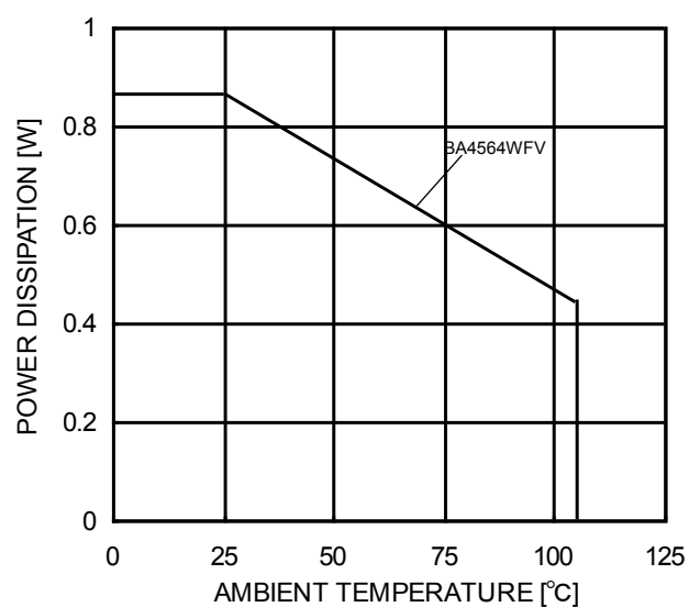
Figure 68. Derating Curve
