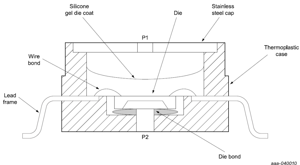
Figure 5. Small outline package — cross-sectional diagram (not to scale)
