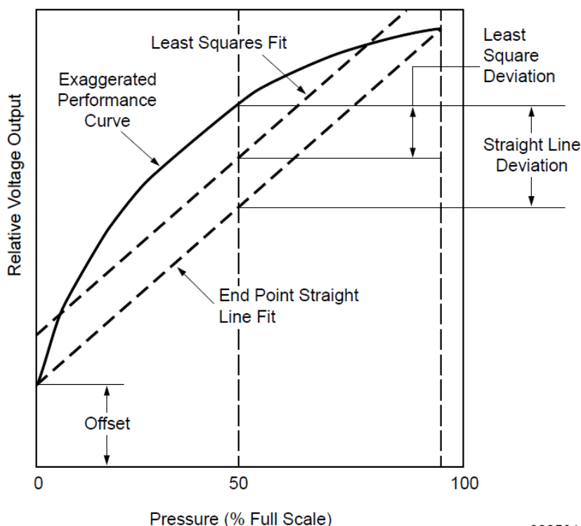
Figure 4. Linearity specification comparison
