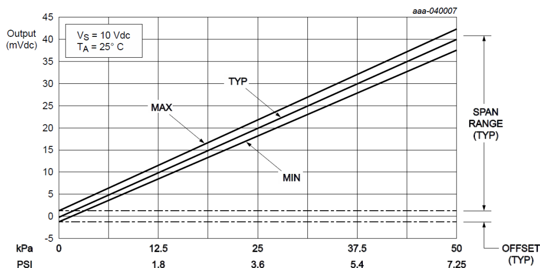
Figure 3. Output vs. pressure differential
