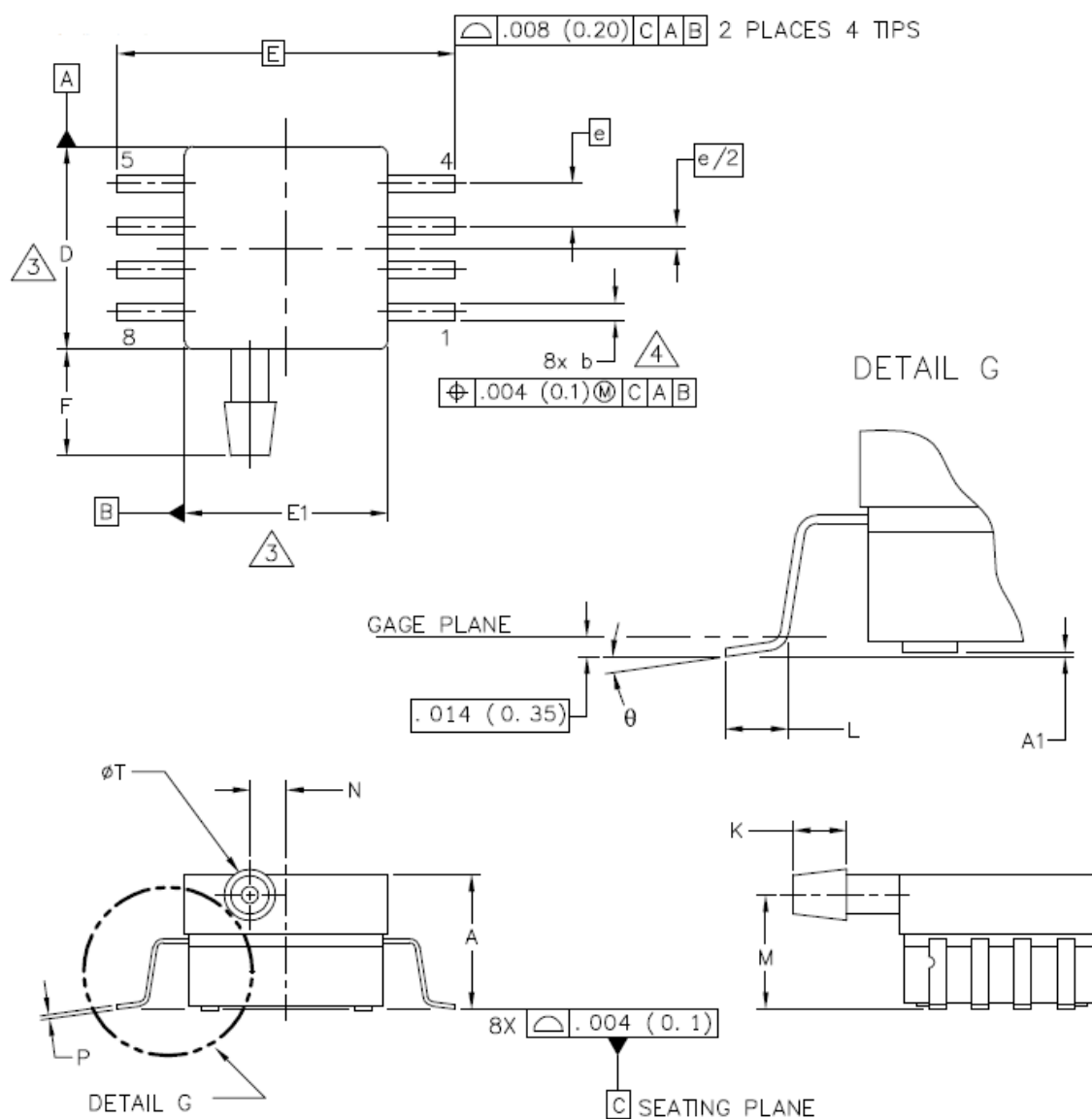
Figure 6. SOT1693-3 (Case 1369-01) – Page 1
