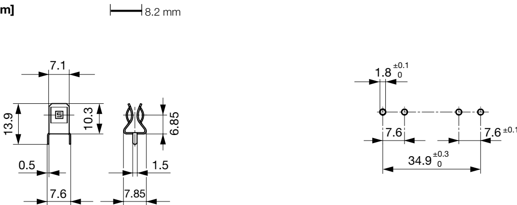
Drilling diagram
