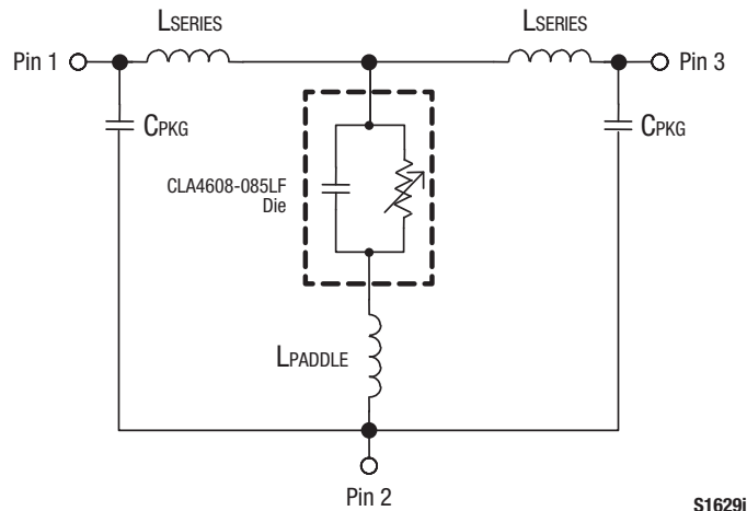
Figure 7. CLA4608-085LF Electrically Equivalent Circuit
