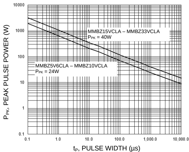
Figure 5. Pulse Rating Curve P_{PK} vs. Pulse Width
