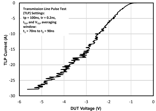
TLP Curve (Negative Pulse)
