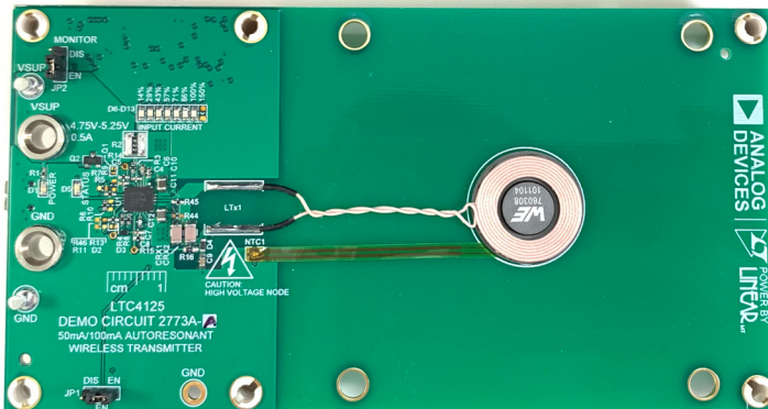
Figure 1. DC2773A-A Picture
