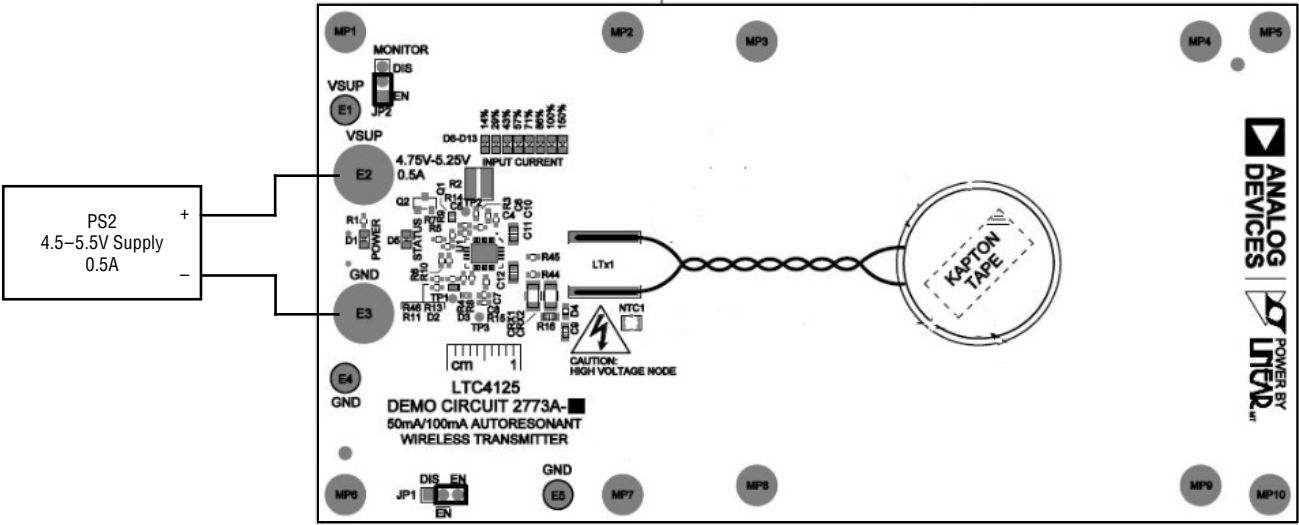
Figure 5. DC2773A-A Top
