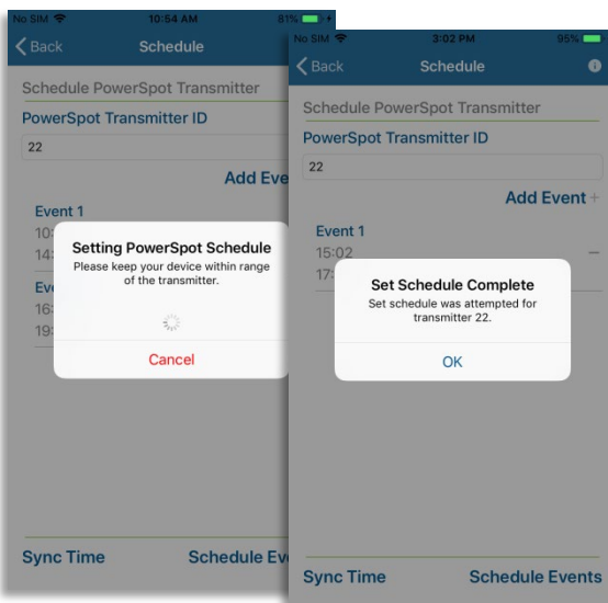
Fig. 6.7– Setting Schedule
