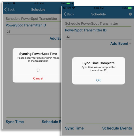
Fig. 6.6– Syncing Time
