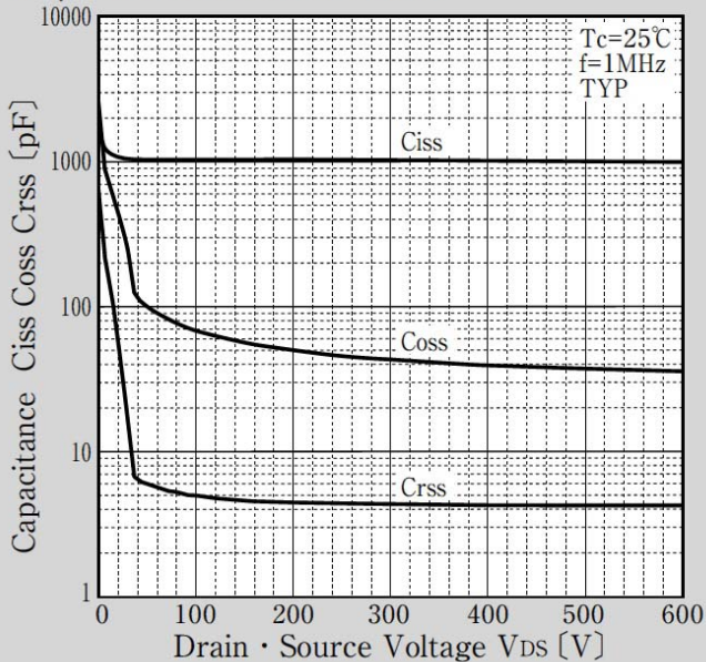
Capacitance Characteristics
