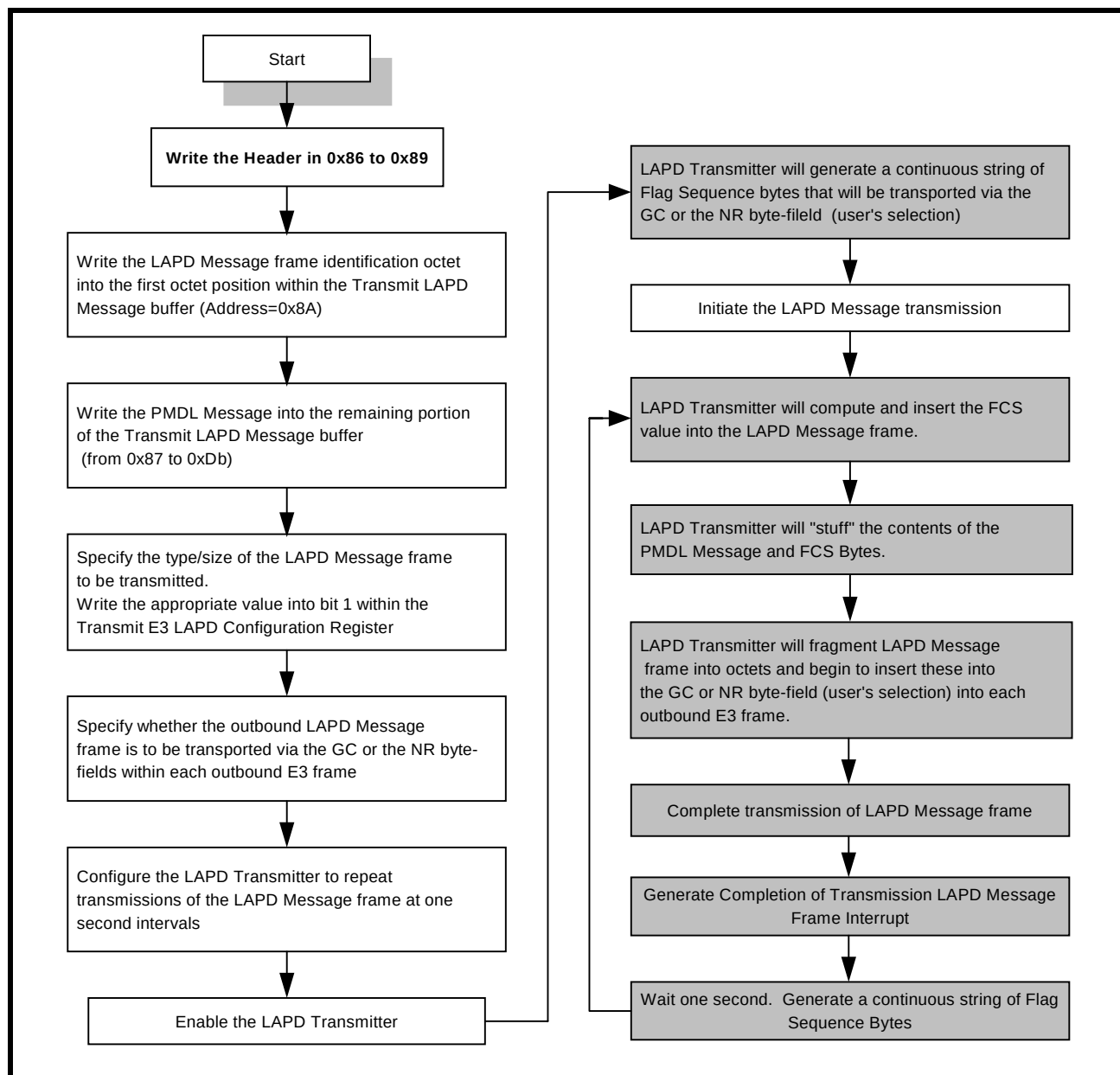
FIGURE 163. FLOW CHART DEPICTING HOW TO USE THE LAPD TRANSMITTER (LAPD TRANSMITTER IS CONFIGURED TO RE-TRANSMIT THE LAPD MESSAGE FRAME REPEATEDLY AT ONE-SECOND INTERVALS)
