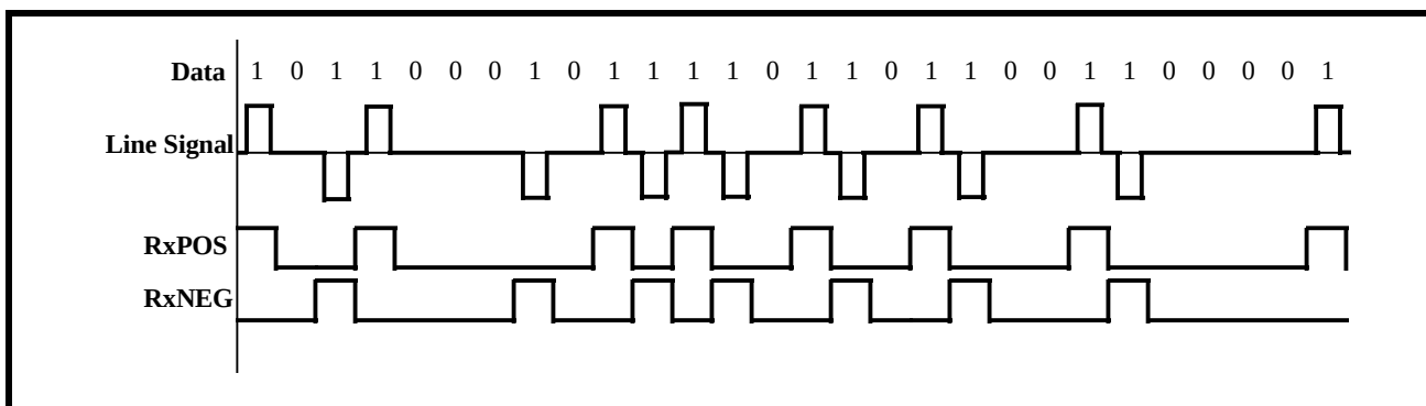
FIGURE 177. ILLUSTRATION OF AMI LINE CODE
