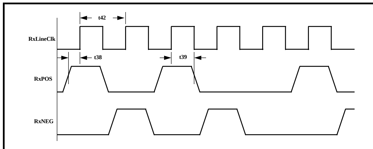
FIGURE 121. WAVEFORM/TIMING RELATIONSHIP BETWEEN RxLineClk, RxPOS AND RxNEG - WHEN RxPOS AND RxNEG ARE TO BE SAMPLED ON THE RISING EDGE OF RxLineClk
