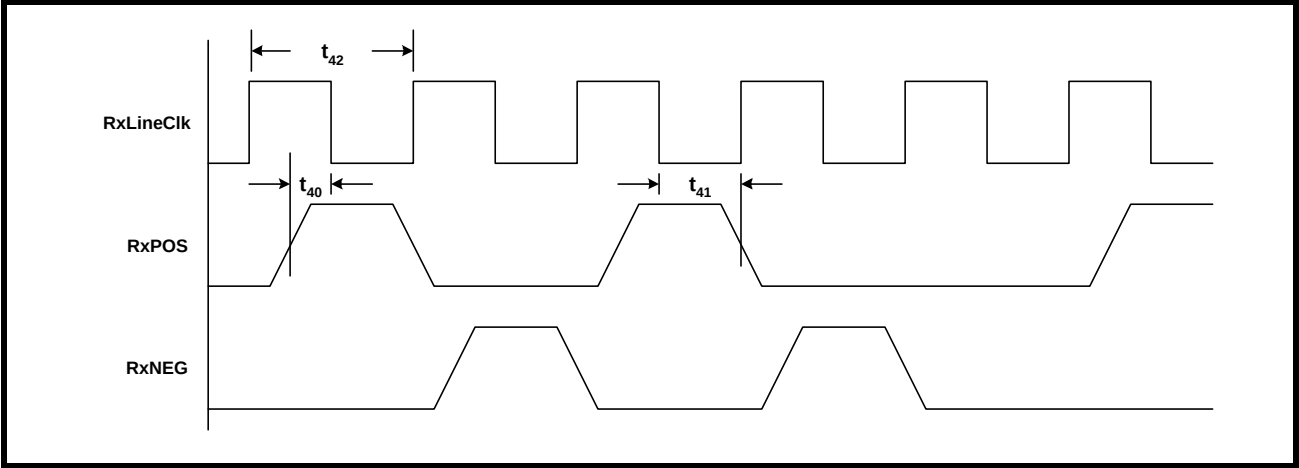
FIGURE 180. WAVEFORM/TIMING RELATIONSHIP BETWEEN RxLineClk, RxPOS AND RxNEG - WHEN RxPOS AND RxNEG ARE TO BE SAMPLED ON THE FALLING EDGE OF RxLineClk
