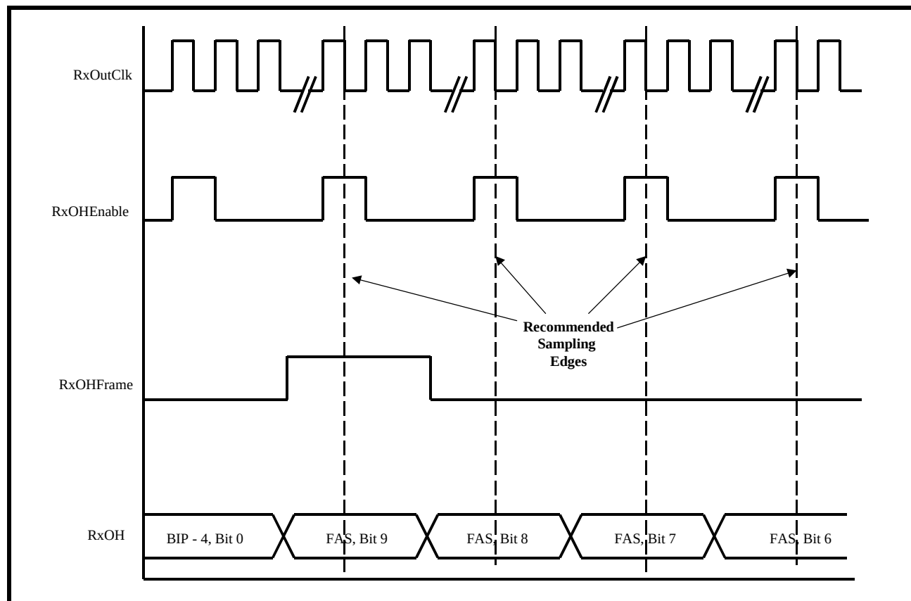
FIGURE 136. ILLUSTRATION OF THE SIGNALS THAT ARE OUTPUT VIA THE RECEIVE OVERHEAD DATA OUTPUT INTERFACE BLOCK (FOR METHOD 2).
