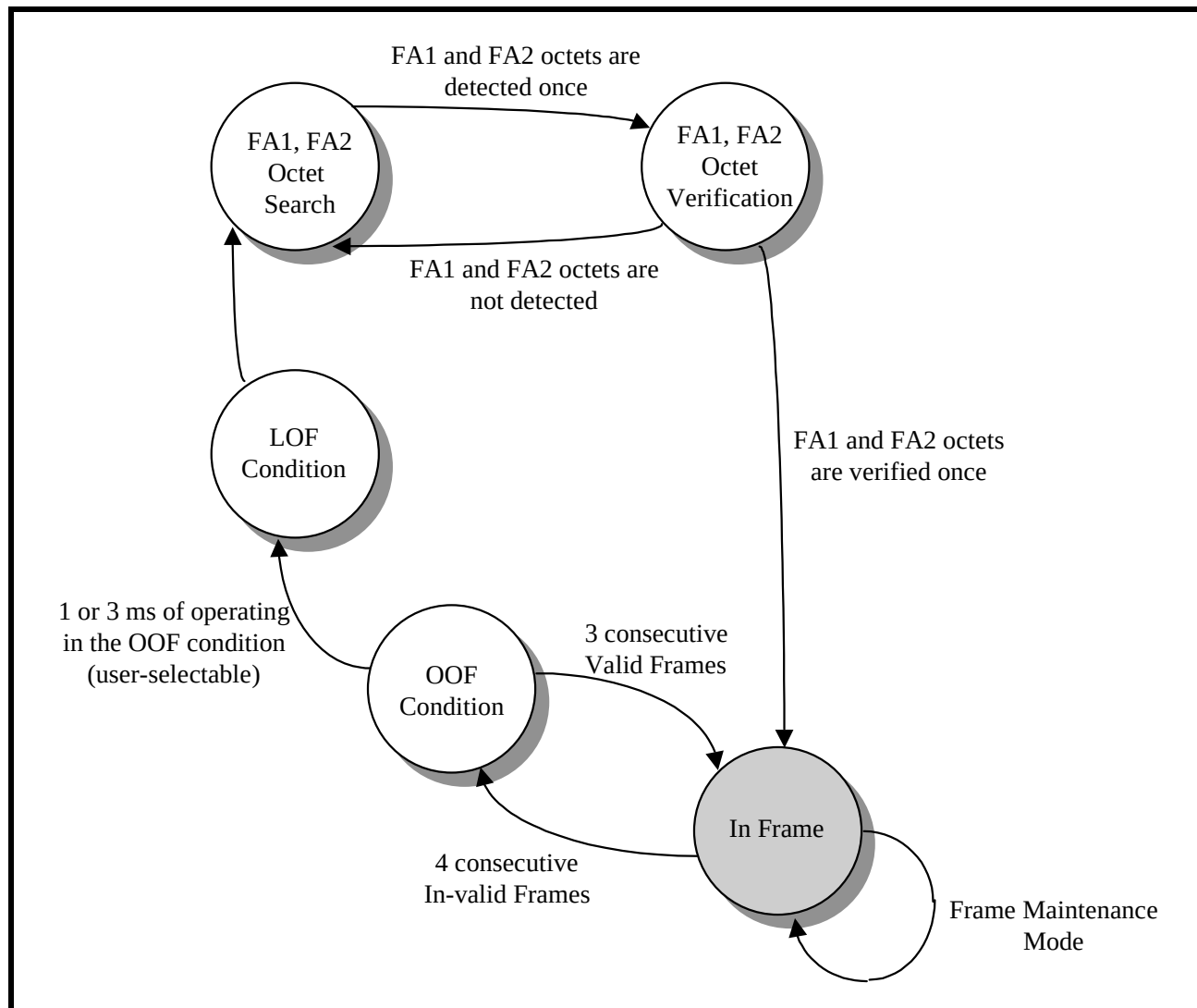
FIGURE 182. THE STATE MACHINE DIAGRAM FOR THE RECEIVE E3 FRAMER E3 FRAME ACQUISITION/MAINTENANCE ALGORITHM
