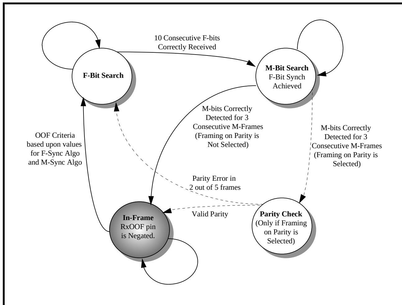
FIGURE 69. THE STATE MACHINE DIAGRAM FOR THE RECEIVE DS3 FRAMER BLOCK'S FRAME ACQUISITION/MAINTENANCE ALGORITHM
