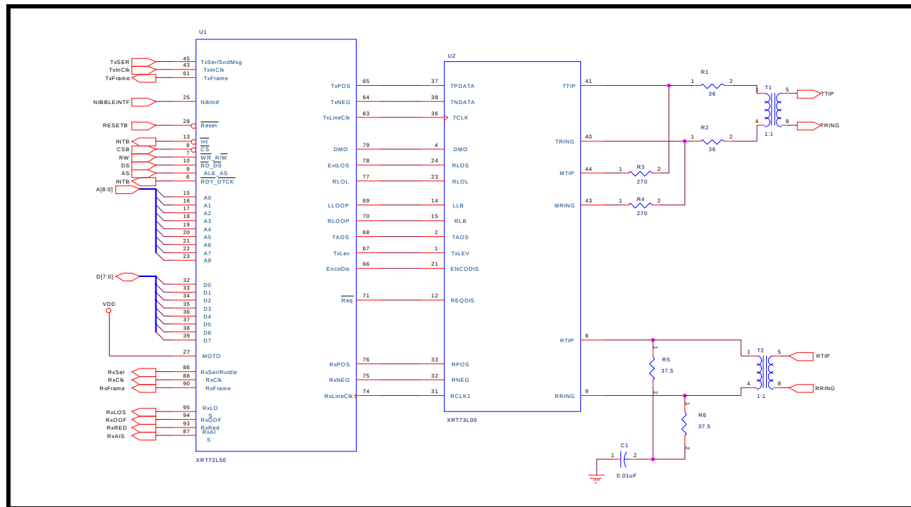
FIGURE 63. IINTERFACING THE XRT72L50 FRAMER IC TO THE XRT73L00 DS3/E3/STS-1 LIU
