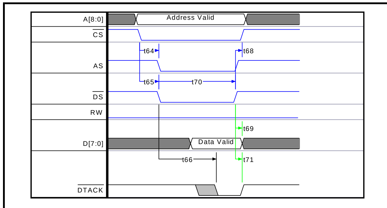
FIGURE 20. MICROPROCESSOR INTERFACE TIMING - MOTOROLA-TYPE PROGRAMMED I/O WRITE OPERATION
