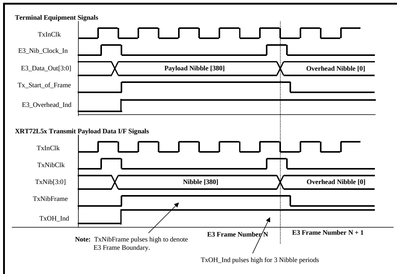
FIGURE 99. BEHAVIOR OF THE TERMINAL INTERFACE SIGNALS BETWEEN THE XRT72L50 AND THE TERMINAL EQUIPMENT (E3 MODE 6 OPERATION)
