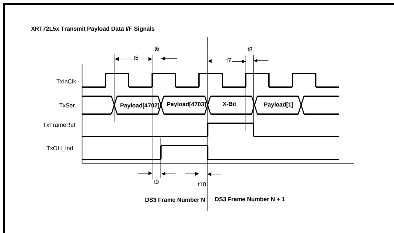
FIGURE 4. TIMING DIAGRAM FOR THE TRANSMIT PAYLOAD INPUT INTERFACE, WHEN THE XRT72L50 DEVICE IS OPERATING IN BOTH THE DS3 AND LOCAL-TIMING MODES
