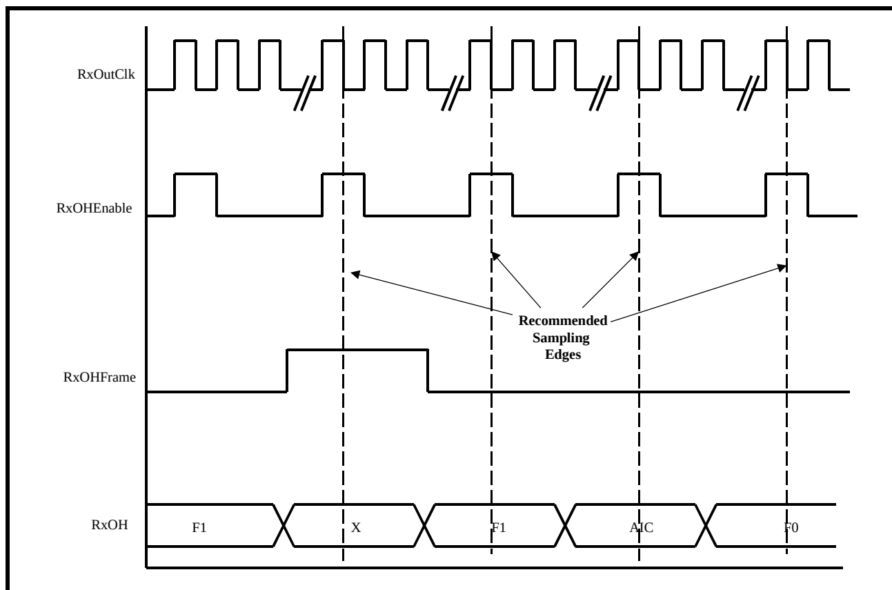
FIGURE 79. ILLUSTRATION OF THE SIGNALS THAT ARE OUTPUT VIA THE RECEIVE OVERHEAD DATA OUTPUT INTERFACE BLOCK (FOR METHOD 2).
