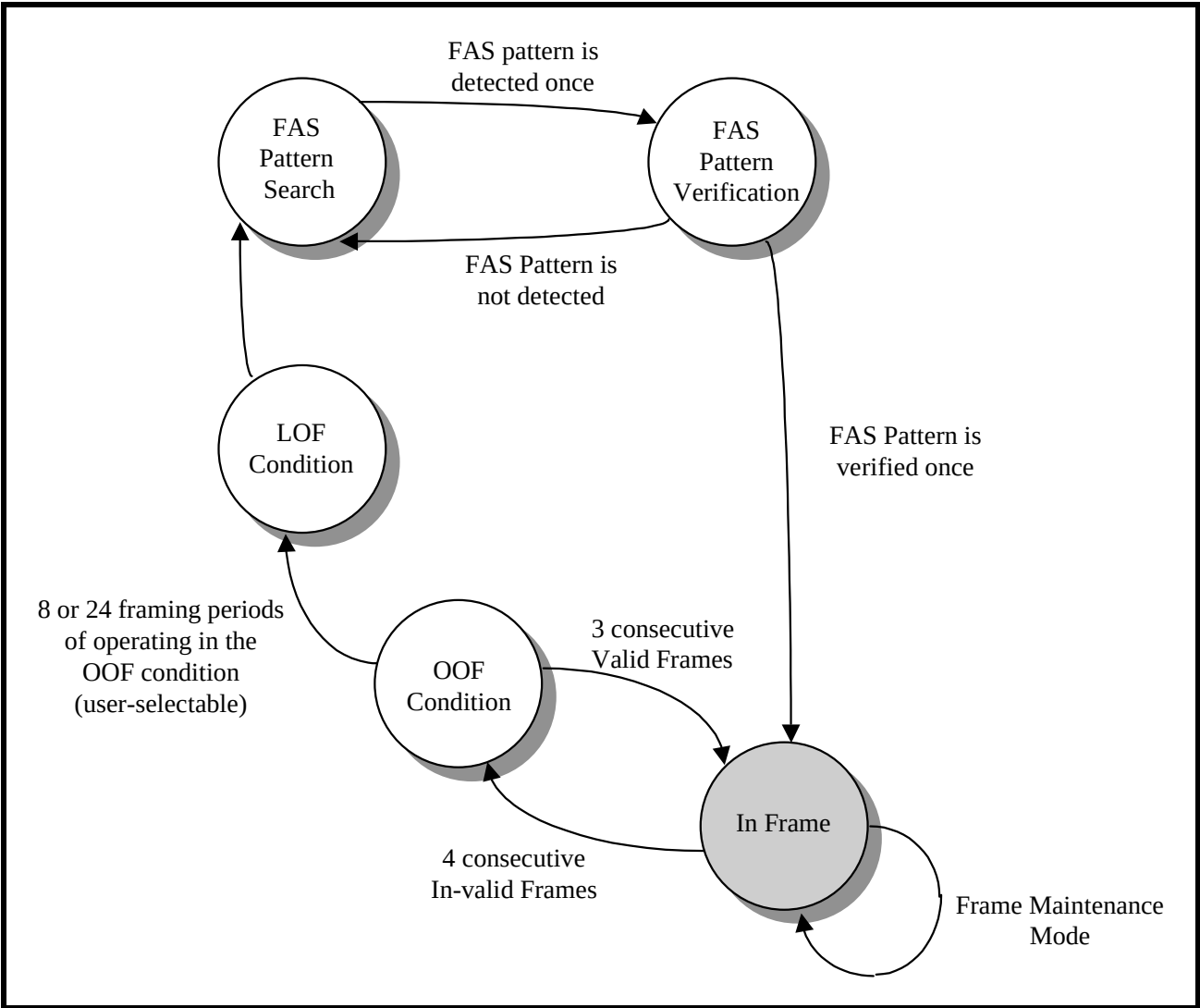
FIGURE 124. THE STATE MACHINE DIAGRAM FOR THE RECEIVE E3 FRAMER E3 FRAME ACQUISITION/MAINTENANCE ALGORITHM
