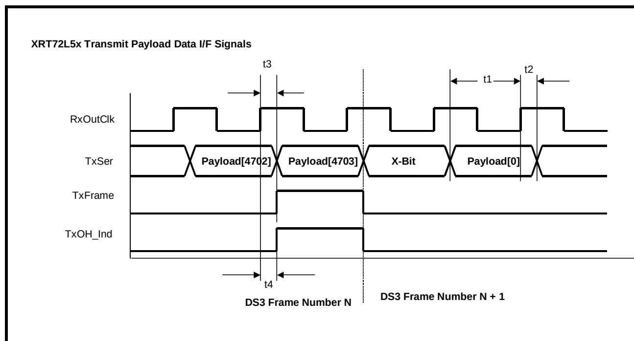
FIGURE 3. TIMING DIAGRAM FOR TRANSMIT PAYLOAD INPUT INTERFACE, WHEN THE XRT72L50 DEVICE IS OPERATING IN BOTH THE DS3 AND LOOP-TIMING MODES
