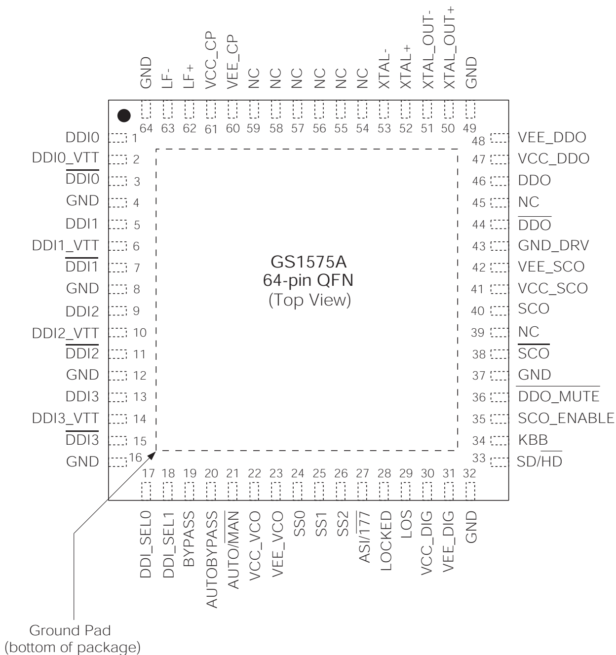
Figure 1-1: 64-Pin QFN
