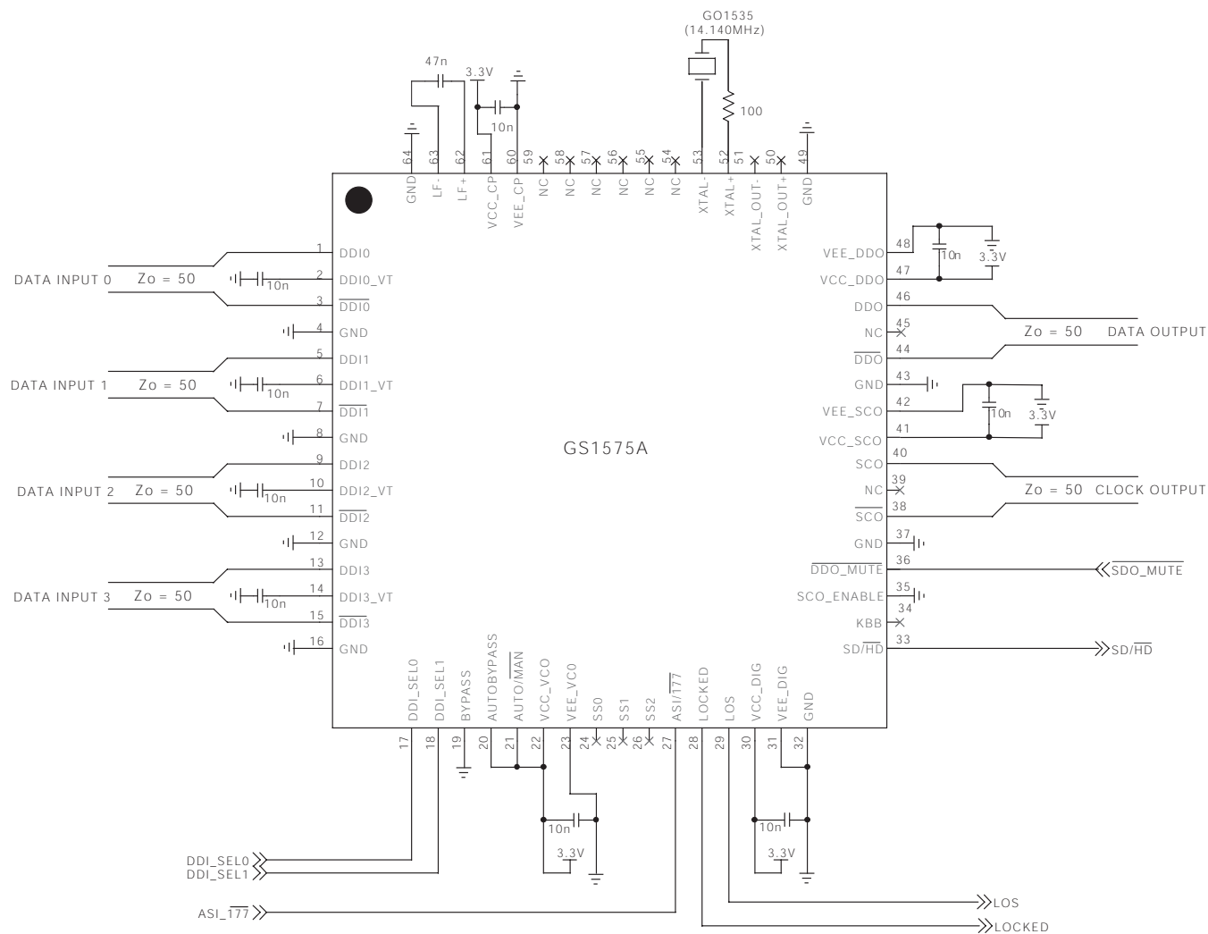
Figure 5-1: GS1575A Typical Application Circuit
