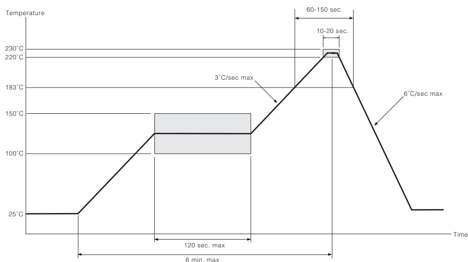
Figure 2-4: Standard Pb Solder Reflow Profile (Pb-free package)
