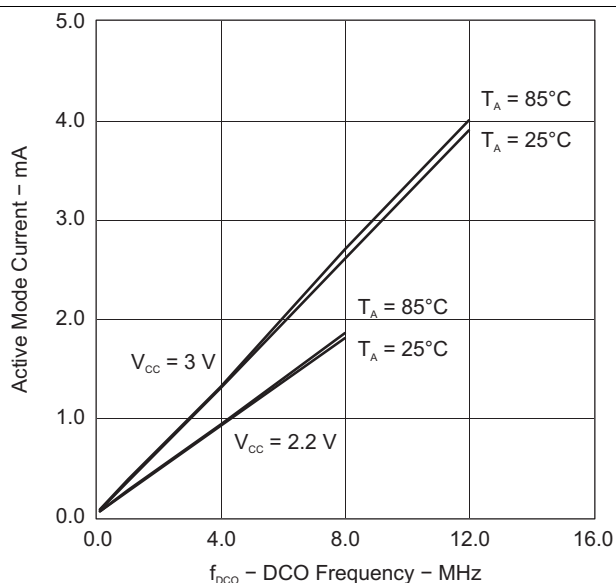
Figure 13. Active-Mode Current vs DCO Frequency
