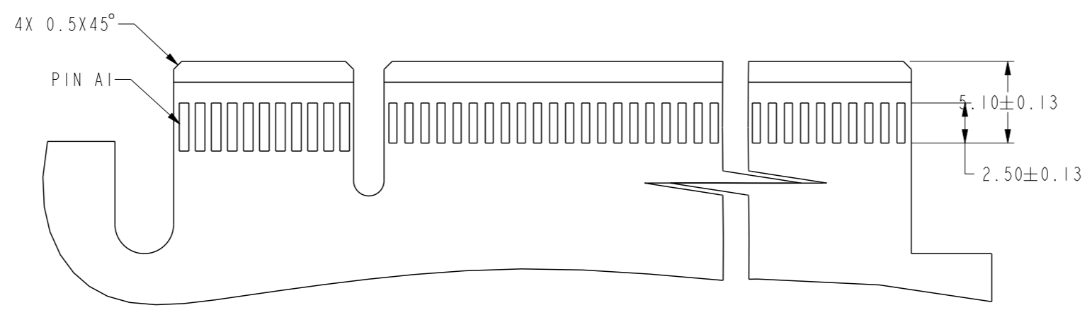
ADD-IN CARD EDGE-FINGER DIMENSIONS SENCONDARY (SOLDER) SIDE (DETAILS : SEE PCIE STRADDLE MOUNT ROUTING GUIDELINE SPEC)
