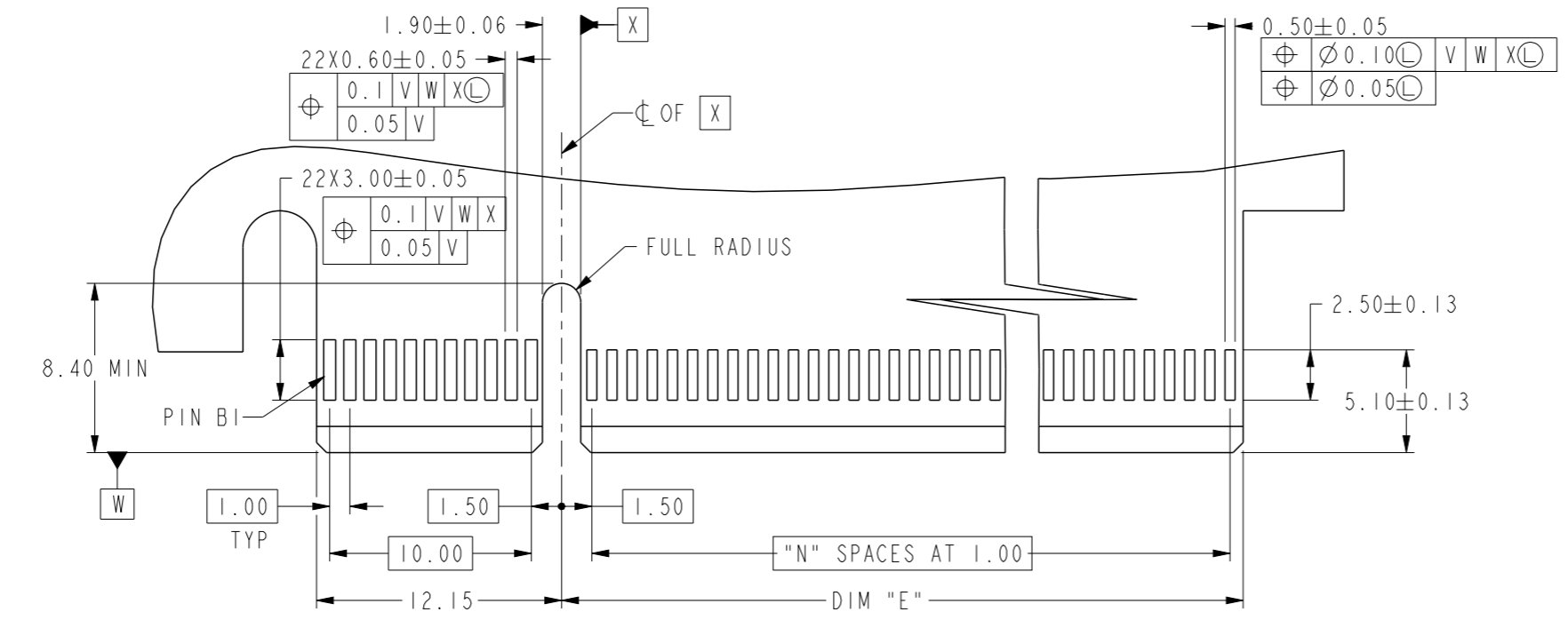
ADD-IN CARD EDGE-FINGER DIMENSIONS PRIMARY (COMPONENT) SIDE (DETAILS : SEE PCIE STRADDLE MOUNT ROUTING GUIDELINE SPEC)
