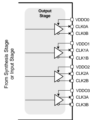
Figure 14. Output Stage
