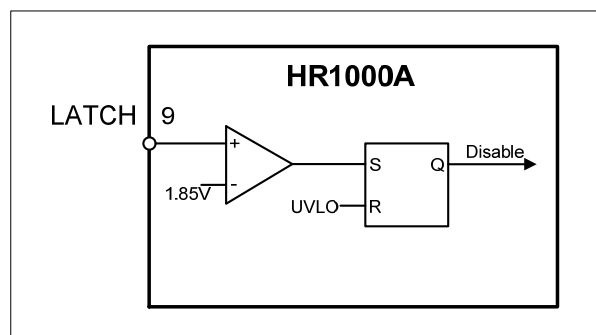
Figure 13: Latch Function Block
