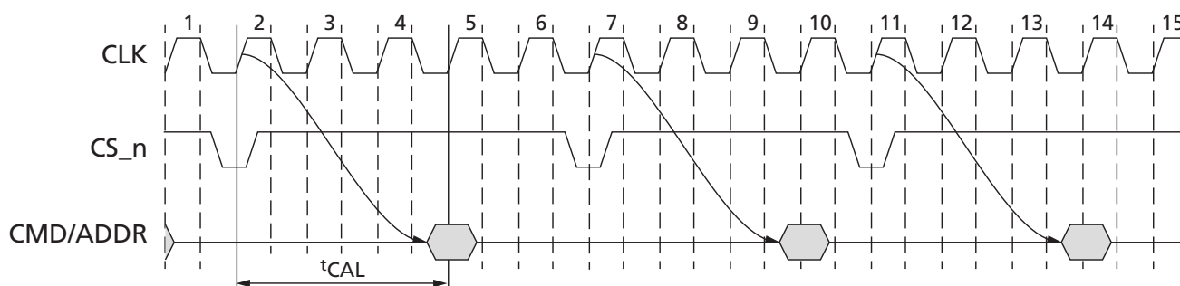
Figure 23: CAL Timing Definition
