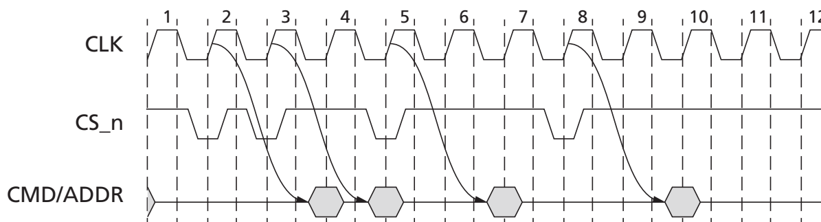
Figure 24: CAL Timing Example (Consecutive \text{CS}_n = \text{LOW} )
