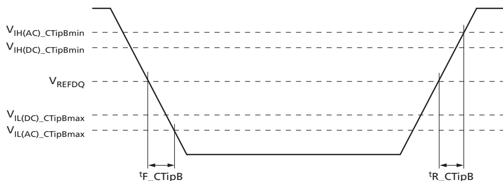
Figure 214: CT Type-B Input Slew Rate Definition
