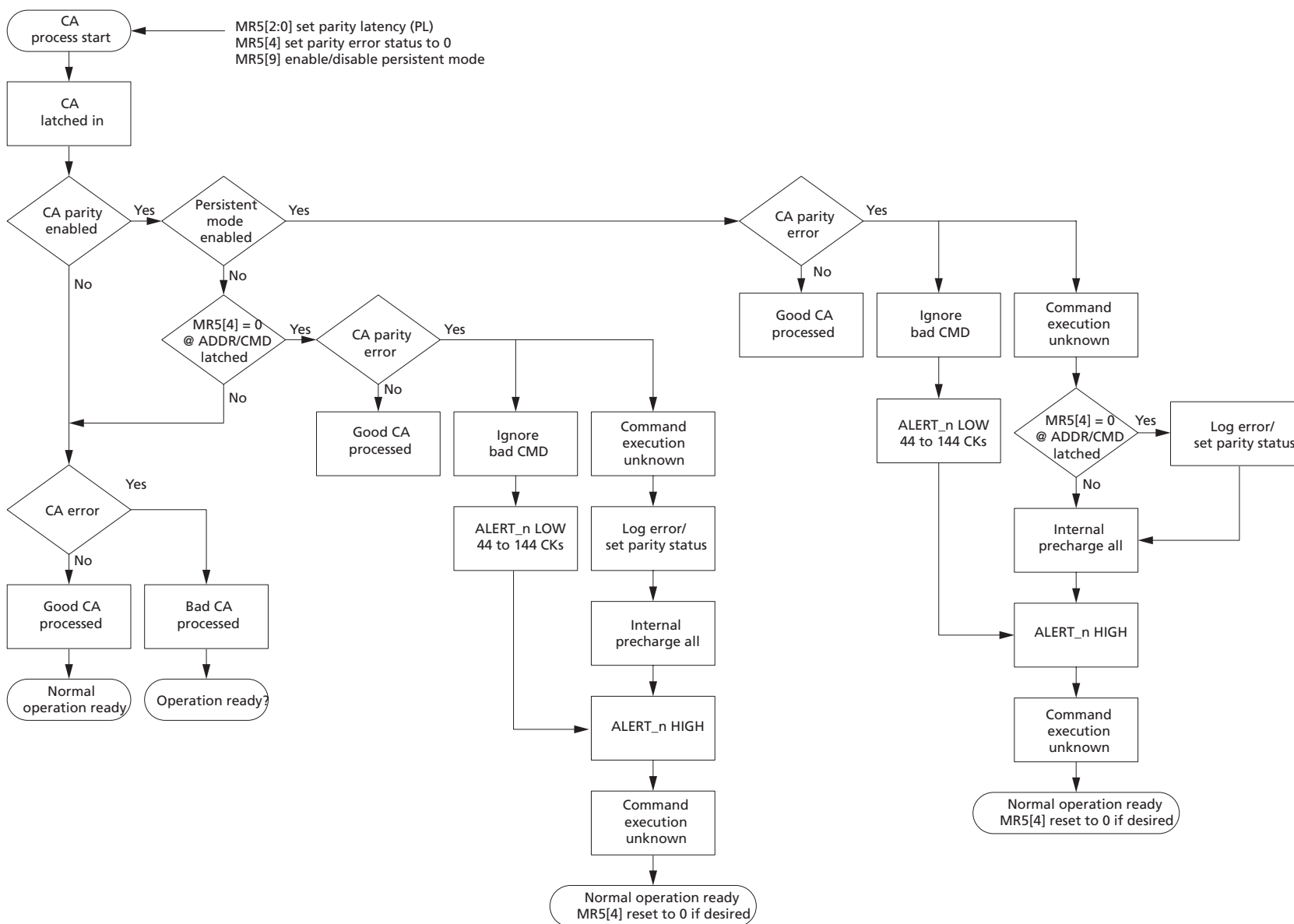
Figure 58: CA Parity Flow Diagram
