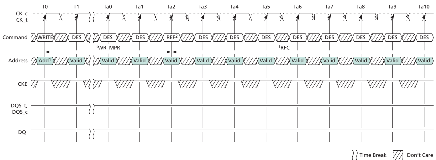
Figure 40: WRITE-to-REFRESH Timing
