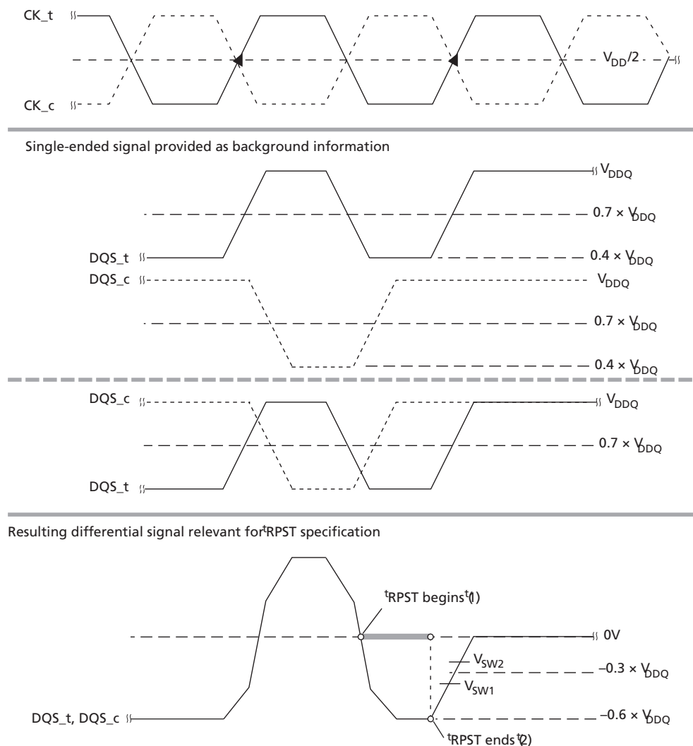
Figure 126: t_{RPST} Method for Calculating Transitions and Endpoints
