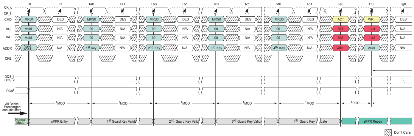
Figure 76: sPPR – Entry
