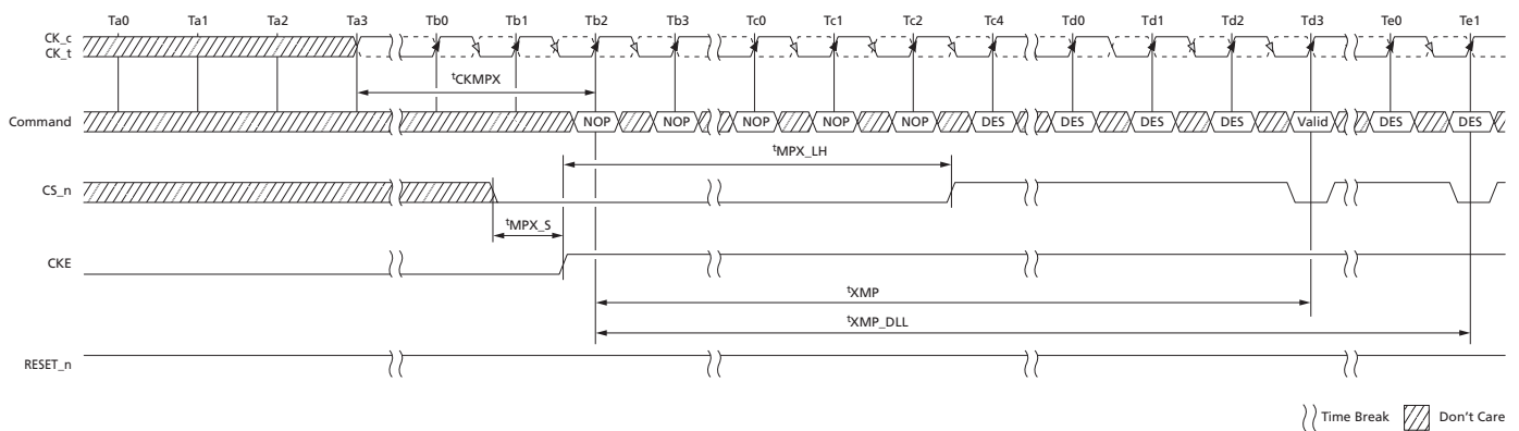
Figure 47: Maximum Power-Saving Mode Exit
