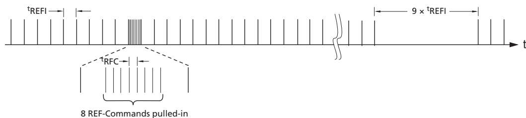
Figure 82: Pulling In REFRESH Commands (Example)
