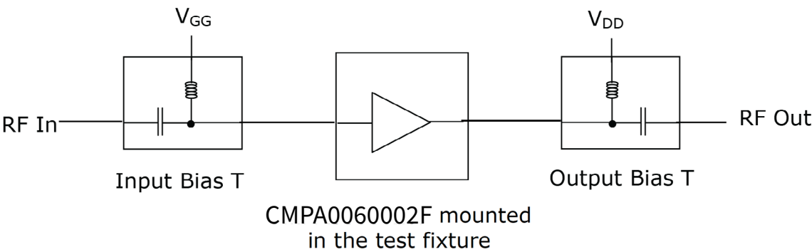
Figure 5. Typical test system setup required for measuring CMPA0060002F-AMP
