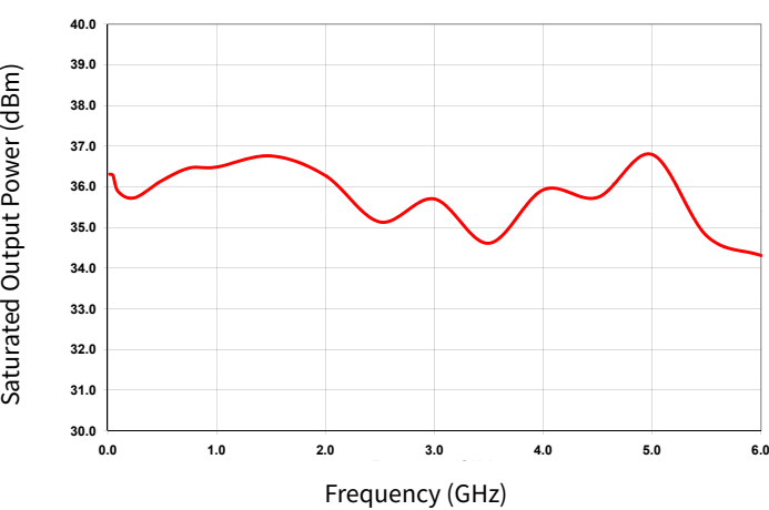
Figure 3. Saturated Output Power Performance ( P_{SAT} ) vs Frequency
