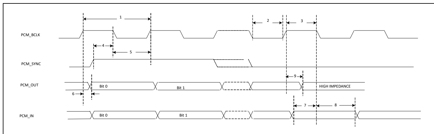
Figure 23. PCM Timing Diagram (Long Frame Sync, Slave Mode)
