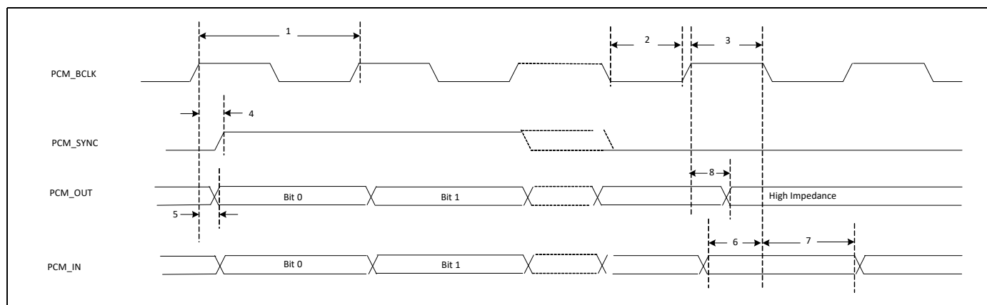
Figure 22. PCM Timing Diagram (Long Frame Sync, Master Mode)
