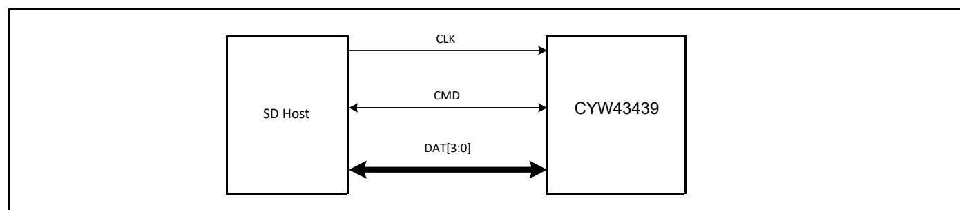
Figure 7. Signal Connections to SDIO Host (SD 4-Bit Mode)
