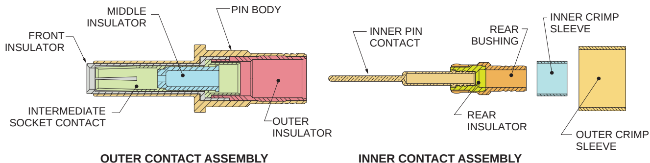
OUTER CONTACT ASSEMBLY
