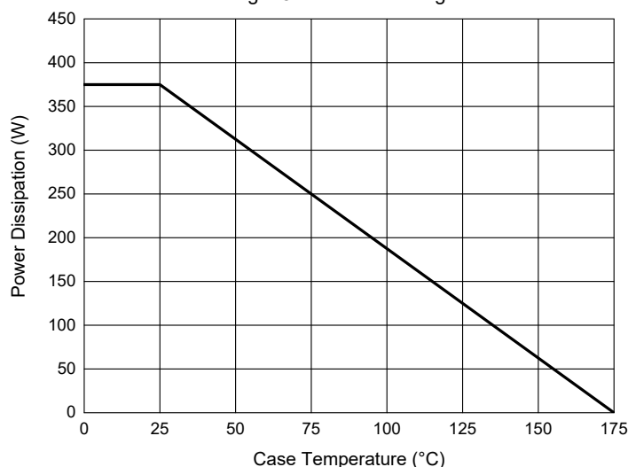
Fig. 18 - Power Derating
