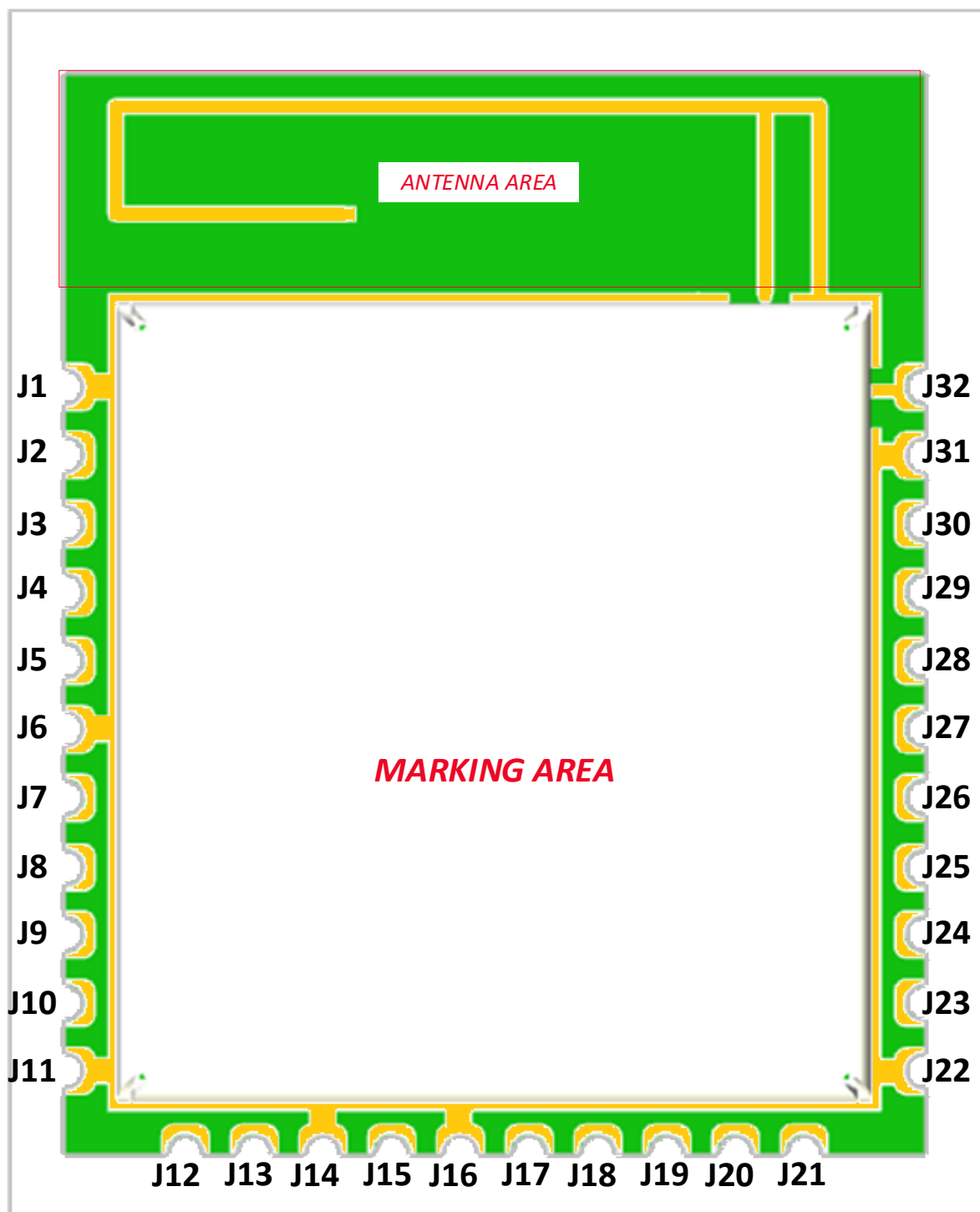
Figure 2. Pinout diagram (top view)
