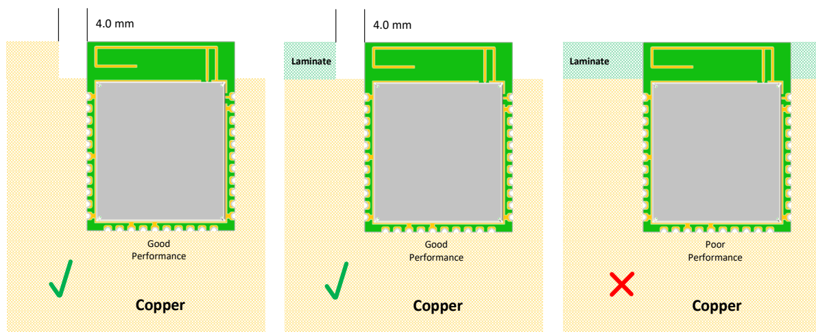
Figure 6. Antenna performance in proximity of copper (left), laminate (middle), and laminate under antenna (right) The actual DA14695MOD evaluation board layout that has been used to conduct measurements is shown in Figure 7 .
