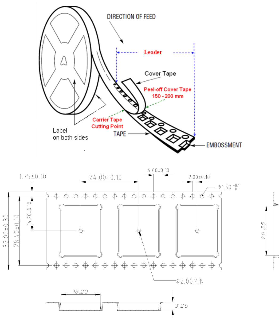
Figure 15. Tape and reel
