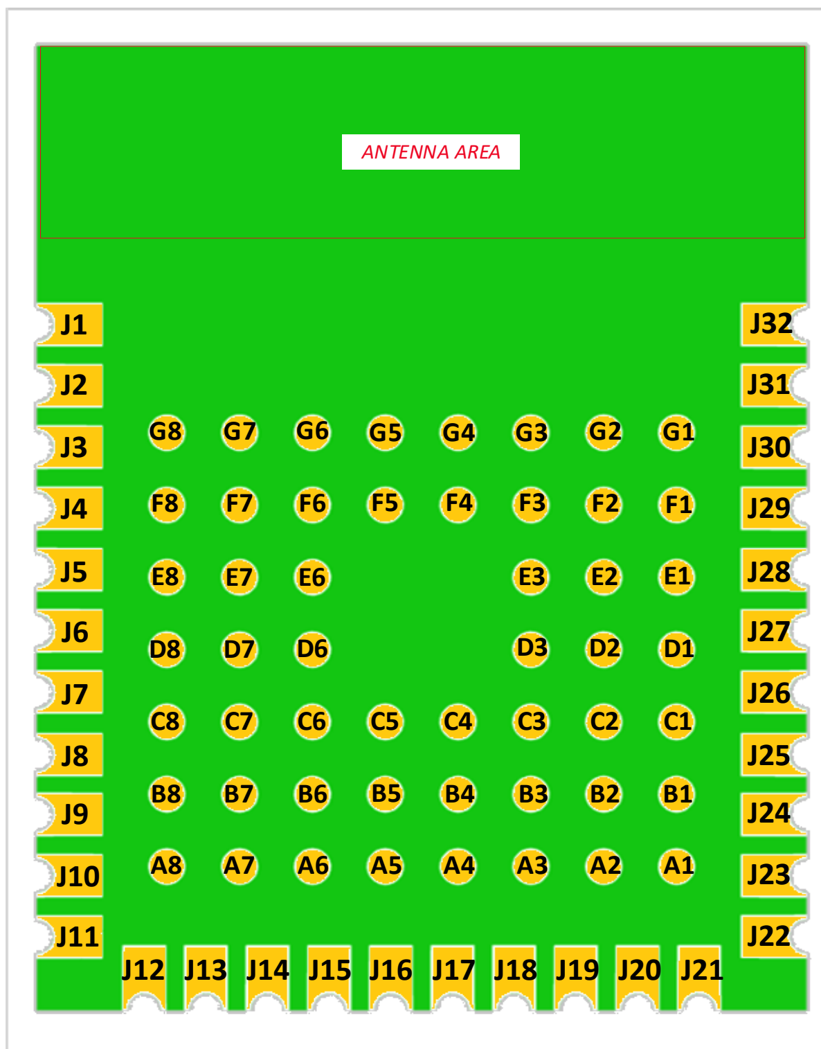
Figure 3. Pinout diagram – bottom pads (top view)
