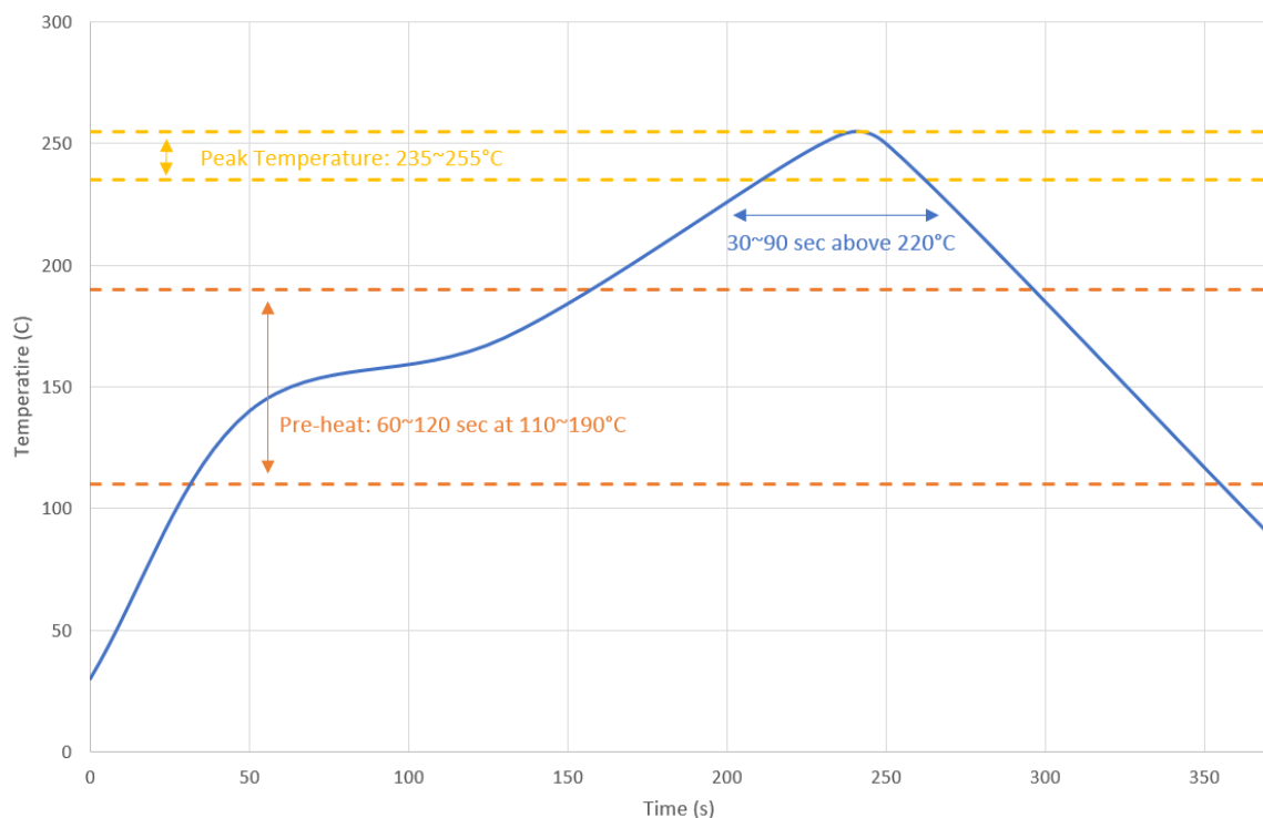
Figure 14. Recommended reflow profile for lead free solder
