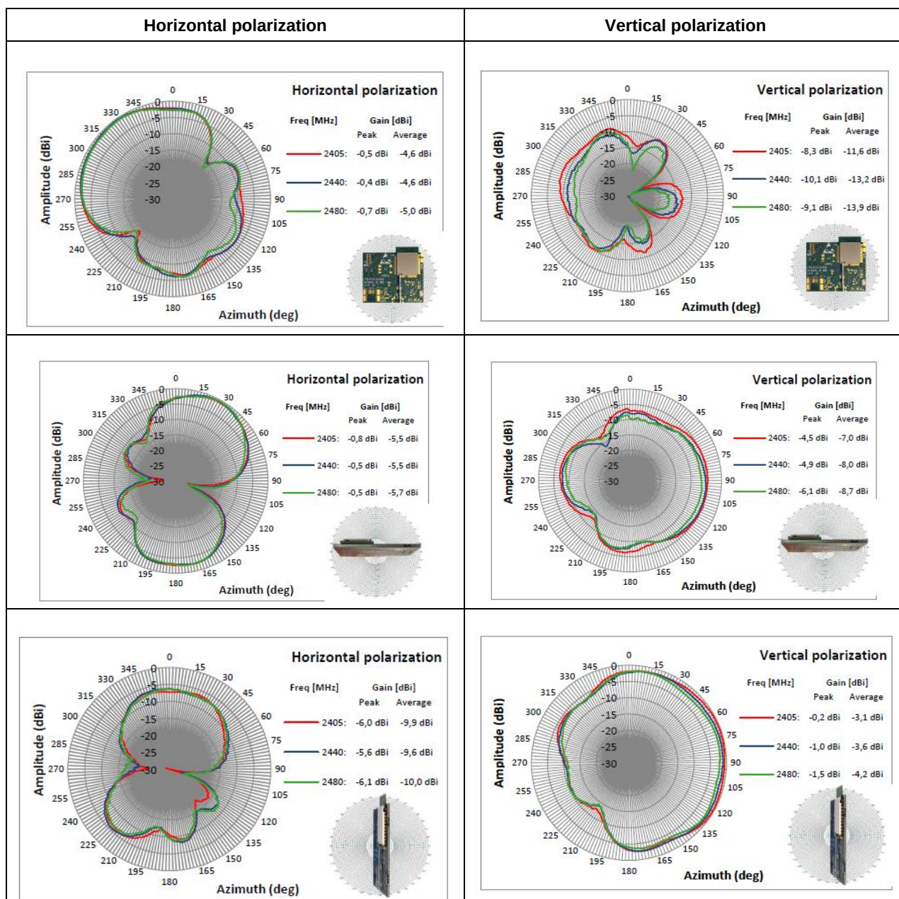
Figure 13. Radiation pattern for trace antenna
