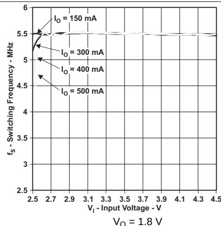
Figure 2. PWM Switching Frequency vs. Input Voltage
