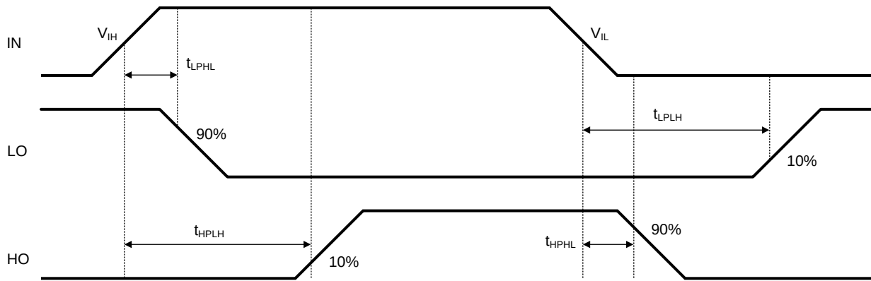
Figure 2. LM5105 Switching Time Definitions: T_{LPLH} , T_{LPHL} , T_{HPLH} , T_{HPLH}
