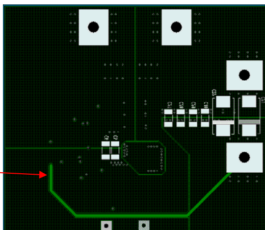
Fig. 25b. IRDC3840 demoboard layout considerations – Bottom Layer
