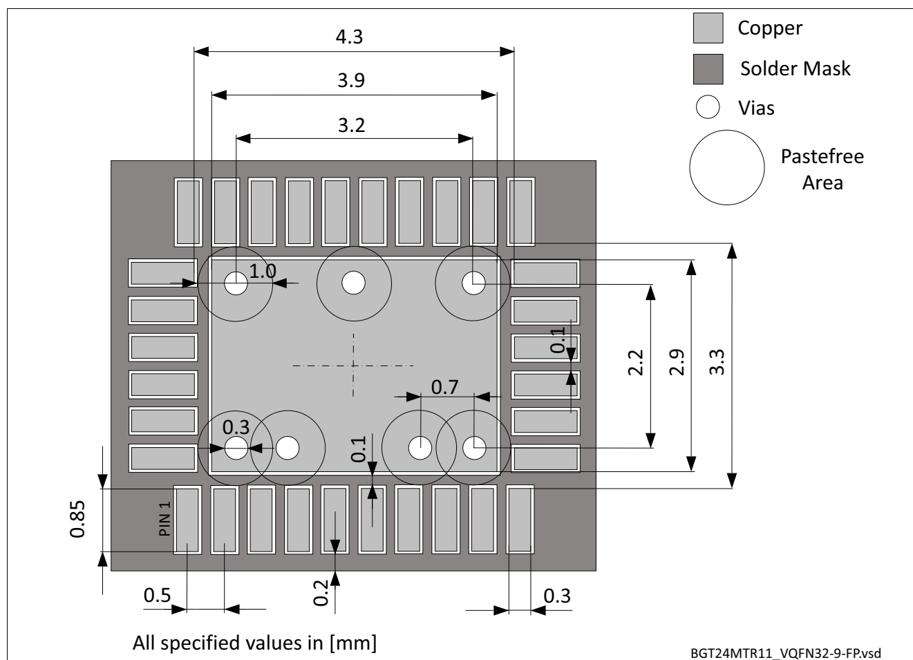
Figure 8 Recommended Footprint and Stencil Layout for the VQFN32-9 Package
