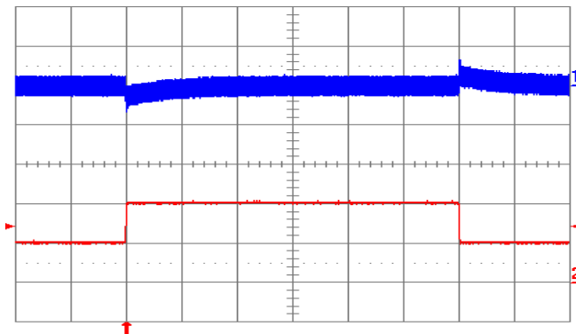
Fig. 12V.11: Output voltage response to load current step-change (1A – 2A – 1A) at V_{in} = 24\text{V} . Top trace: output voltage (200 mV/div.). Bottom trace: load current (1 A/div.). Current slew rate: 0.1 A/µs. C_o = 1\text{ }\mu\text{F} ceramic. Time scale: 0.5 ms/div.
