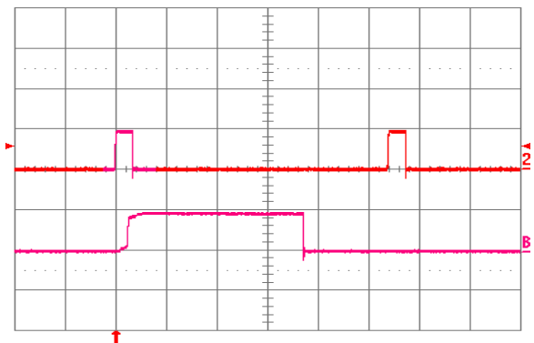
Fig. 1.0V.18: Load current (top trace, 20 A/div., 20 ms/div.) into a 10\ \text{m}\Omega short circuit during restart, at V_{in} = 24\ \text{V} . Bottom trace (20 A/div., 2 ms/div.) is an expansion of the on-time portion of the top trace.
