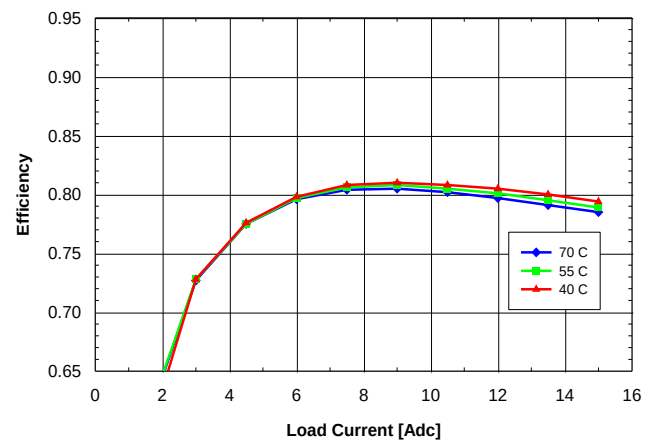
Fig. 1.0V.6: Efficiency vs. load current and ambient temperature for SQ24T/S15010 converter mounted vertically with V_{in} = 24V and air flowing from pin 3 to pin 1 at a rate of 200 LFM (1.0 m/s).
