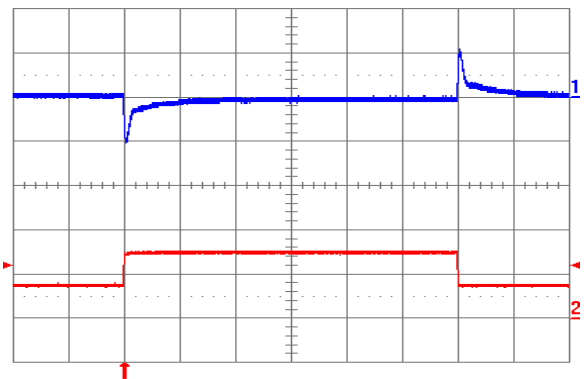
Fig. 1.8V.12: Output voltage response to load current step-change (3.75A – 7.5A – 3.75A) at V_{in} = 24\text{V} . Top trace: output voltage (100 mV/div.). Bottom trace: load current (5 A/div.). Current slew rate: 5 A/µs. C_o = 450\text{ }\mu\text{F} tantalum + 1 µF ceramic. Time scale: 0.2 ms/div.
