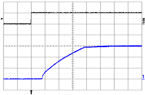
Fig. 6.0V.10: Turn-on transient at full rated load current (resistive) plus 10,000 µF at V_{in} = 24\text{V} , triggered via ON/OFF pin. Top trace: ON/OFF signal (5 V/div.). Bottom trace: output voltage (2 V/div.). Time scale: 2 ms/div.
