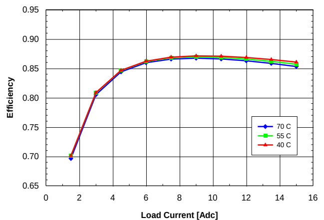
Fig. 2.5V.6: Efficiency vs. load current and ambient temperature for SQ24T/S15025 converter mounted vertically with V_{in} = 24V and air flowing from pin 3 to pin 1 at a rate of 200 LFM (1.0 m/s).
