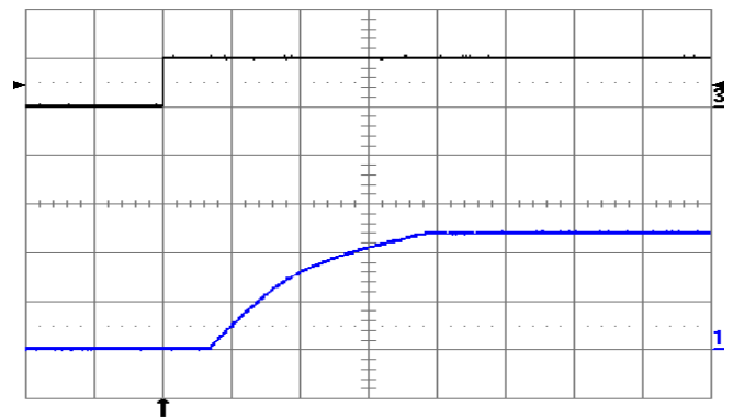
Fig. 12V.10: Turn-on transient at full rated load current (resistive) plus 1,000µF at V_{in} = 24\text{V} , triggered via ON/OFF pin. Top trace: ON/OFF signal (5 V/div.). Bottom trace: output voltage (5 V/div.). Time scale: 2 ms/div.
