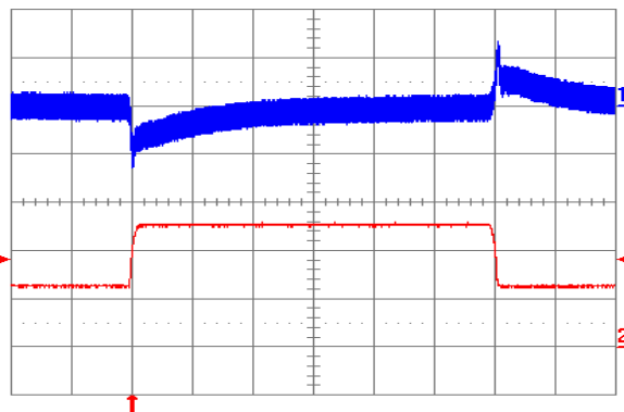
Fig. 5.0V.11: Output voltage response to load current step-change (2.5A – 5A – 2.5A) at V_{in} = 24\text{V} . Top trace: output voltage (100 mV/div.). Bottom trace: load current (2 A/div.). Current slew rate: 0.1\text{ A}/\mu\text{s} . C_o = 1\text{ }\mu\text{F} ceramic. Time scale: 0.2 ms/div.
