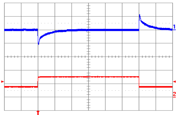
Fig. 2.5V.12: Output voltage response to load current step-change (3.75 A – 7.5 A – 3.75 A) at V_{in} = 24\text{V} . Top trace: output voltage (100 mV/div.). Bottom trace: load current (5 A/div.). Current slew rate: 5 A/ \mu\text{s} . C_o = 450 \mu\text{F} tantalum + 1 \mu\text{F} ceramic. Time scale: 0.2 ms/div.
