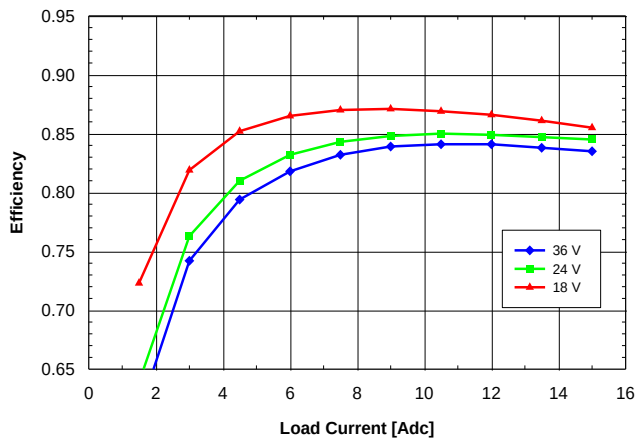
Fig. 1.8V.5: Efficiency vs. load current and input voltage for SQ24T/S15018 converter mounted vertically with air flowing from pin 3 to pin 1 at a rate of 300 LFM (1.5 m/s) and T_a = 25^{\circ}C .
