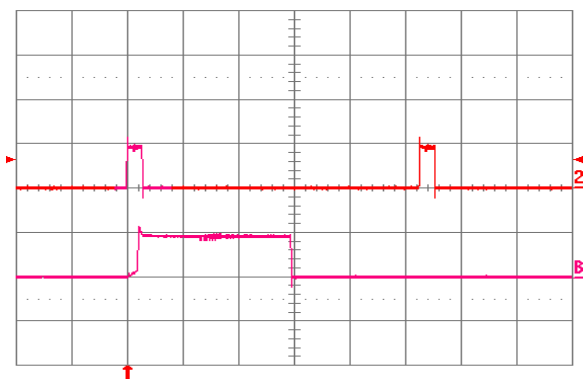
Fig. 1.8V.18: Load current (top trace, 20 A/div., 20 ms/div.) into a 10\ \text{m}\Omega short circuit during restart, at V_{in} = 24\ \text{V} . Bottom trace (20 A/div., 2 ms/div.) is an expansion of the on-time portion of the top trace.
