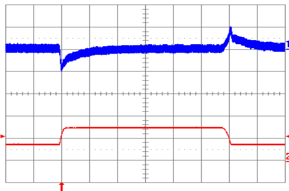
Fig. 3.3V.11: Output voltage response to load current step-change (3.75A – 7.5A – 3.75A) at V_{in} = 24\text{V} . Top trace: output voltage (100 mV/div.). Bottom trace: load current (5 A/div.). Current slew rate: 0.1 A/ \mu\text{s} . C_o = 1 \mu\text{F} ceramic. Time scale: 0.2 ms/div.
