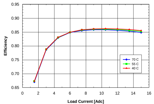
Fig. 2.0V.6: Efficiency vs. load current and ambient temperature for SQ24T/S15020 converter mounted vertically with V_{in} = 24V and air flowing from pin 3 to pin 1 at a rate of 200 LFM (1.0 m/s).
