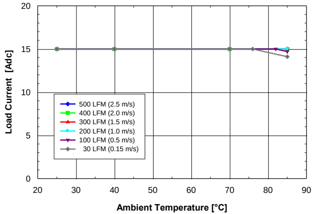
Fig. 1.5V.3: Available load current vs. ambient temperature and airflow rates for SQ24S15015 converter mounted vertically with V_{in} = 24V , air flowing from pin 3 to pin 1 and maximum FET temperature \leq 120^{\circ}C .
