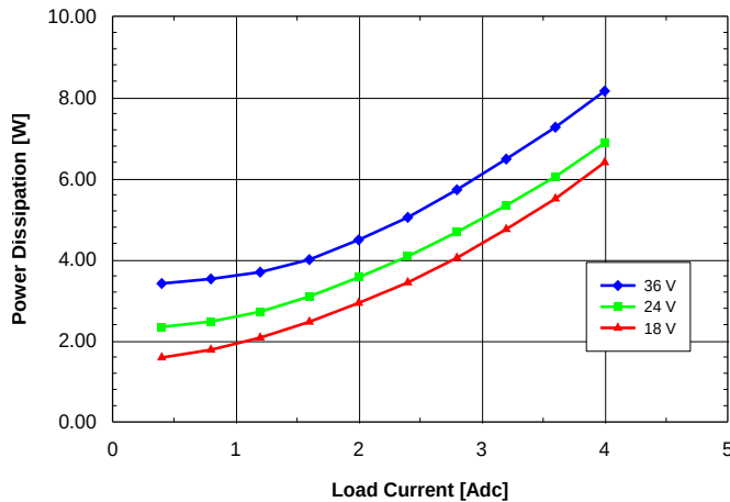
Fig. 12V.7: Power dissipation vs. load current and input voltage for SQ24T/S04120 converter mounted vertically with air flowing from pin 3 to pin 1 at a rate of 300 LFM (1.5 m/s) and T_a = 25^\circ\text{C} .
