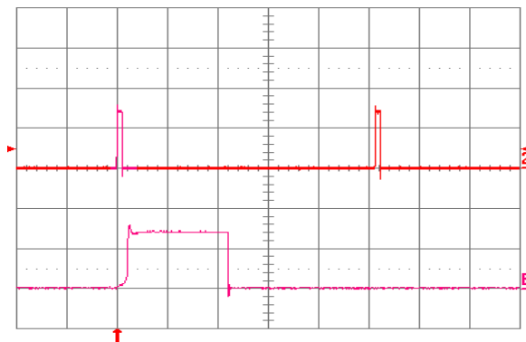
Fig. 5.0V.18: Load current (top trace, 10 A/div., 20 ms/div.) into a 10\ \text{m}\Omega short circuit during restart, at V_{in} = 24\ \text{V} . Bottom trace (10 A/div., 1 ms/div.) is an expansion of the on-time portion of the top trace.
