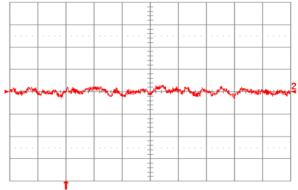
Fig. 1.5V.16: Input reflected ripple current, i_s (10 mA/div.), measured through 10\ \mu\text{H} at the source at full rated load current and V_{in} = 24\ \text{V} . Refer to Fig. 1.5V.14 for test setup. Time scale: 1\ \mu\text{s}/\text{div} .
