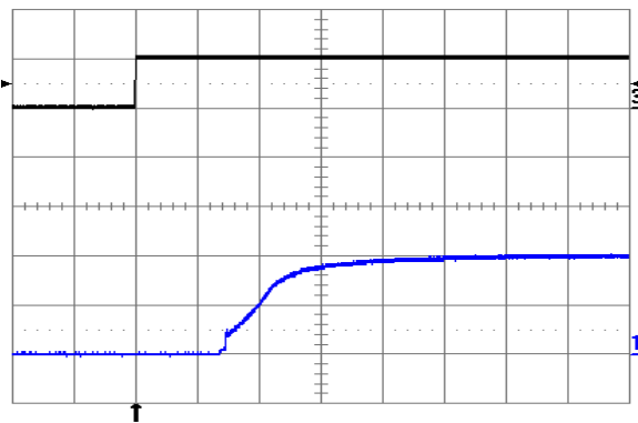
Fig. 2.0V.9: Turn-on transient at full rated load current (resistive) with no output capacitor at V_{in} = 24\text{V} , triggered via ON/OFF pin. Top trace: ON/OFF signal (5 V/div.). Bottom trace: output voltage (1 V/div.). Time scale: 1 ms/div.
