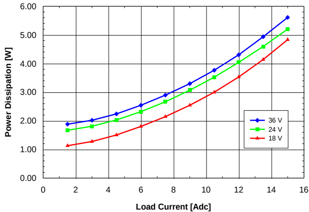
Fig. 2.0V.7: Power dissipation vs. load current and input voltage for SQ24T/S15020 converter mounted vertically with air flowing from pin 3 to pin 1 at a rate of 300 LFM (1.5 m/s) and T_a = 25^\circ\text{C} .
