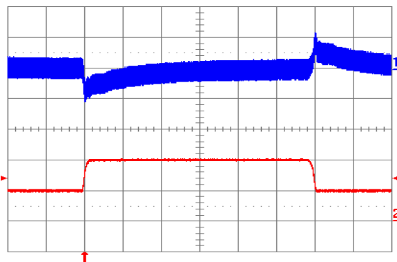
Fig. 6.0V.11: Output voltage response to load current step-change (2A – 4A – 2A) at V_{in} = 24\text{V} . Top trace: output voltage (100 mV/div.). Bottom trace: load current (2 A/div.). Current slew rate: 0.1 A/µs. C_o = 1\text{ }\mu\text{F} ceramic. Time scale: 0.2 ms/div.
