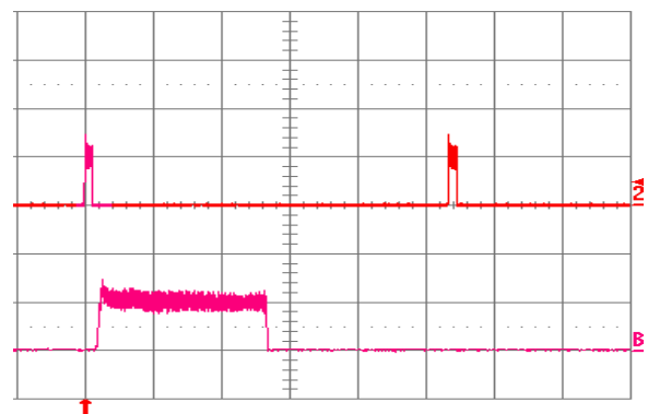
Fig. 12V.18: Load current (top trace, 5 A/div., 20 ms/div.) into a 10\ \text{m}\Omega short circuit during restart, at V_{in} = 24\ \text{V} . Bottom trace (5 A/div., 1 ms/div.) is an expansion of the on-time portion of the top trace.
