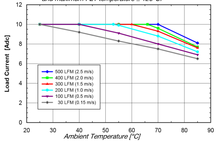
Fig. 5.0V.4: Available load current vs. ambient temperature and airflow rates for SQ24S10050 converter mounted horizontally with V_{in} = 24V , air flowing from pin 3 to pin 1 and maximum FET temperature \leq 120^{\circ}C .
