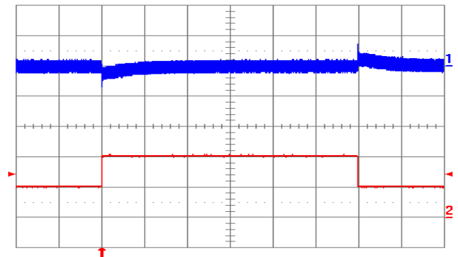
Fig. 12V.12: Output voltage response to load current step-change (1A – 2A – 1A) at V_{in} = 24\text{V} . Top trace: output voltage (200 mV/div.). Bottom trace: load current (1 A/div.). Current slew rate: 5 A/µs. C_o = 1\text{ }\mu\text{F} ceramic. Time scale: 0.5 ms/div.
