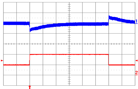
Fig. 6.0V.12: Output voltage response to load current step-change (2A – 4A – 2A) at V_{in} = 24\text{V} . Top trace: output voltage (100 mV/div.). Bottom trace: load current (2 A/div.). Current slew rate: 5 A/µs. C_o = 450\text{ }\mu\text{F} tantalum + 1 µF ceramic. Time scale: 0.2 ms/div.
