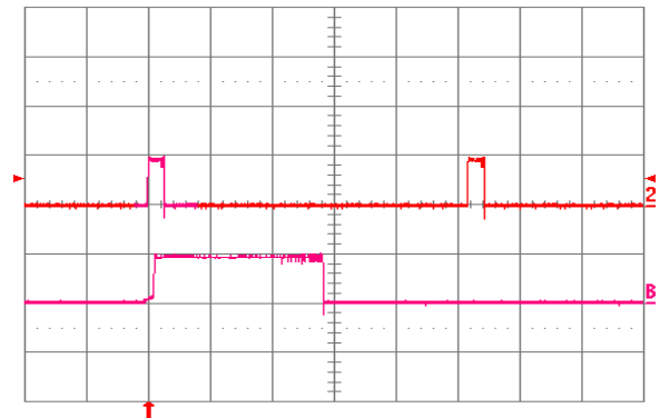
Fig. 2.0V.18: Load current (top trace, 20 A/div., 20 ms/div.) into a 10\ \text{m}\Omega short circuit during restart, at V_{in} = 24\ \text{V} . Bottom trace (20 A/div., 2 ms/div.) is an expansion of the on-time portion of the top trace.
