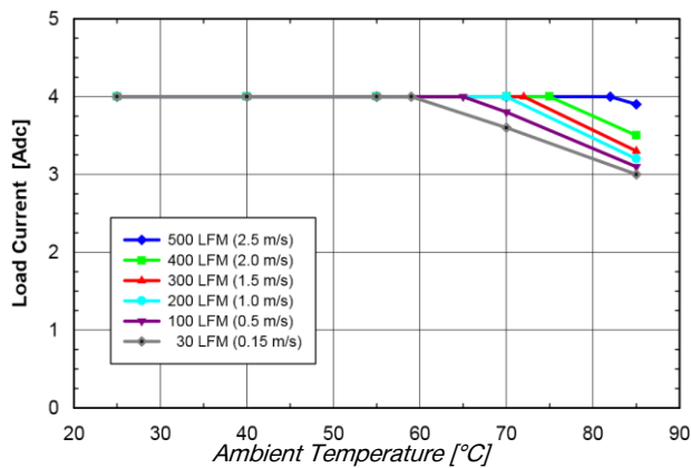
Fig. 12V.3: Available load current vs. ambient temperature and airflow rates for SQ24S04120 converter mounted vertically with V_{in} = 24V , air flowing from pin 3 to pin 1 and maximum FET temperature \leq 120^{\circ}C .
