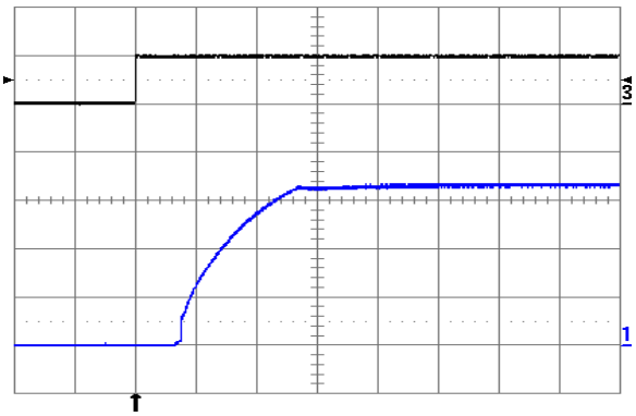
Fig. 3.3V.10: Turn-on transient at full rated load current (resistive) plus 10,000 \mu\text{F} at V_{in} = 24\text{V} , triggered via ON/OFF pin. Top trace: ON/OFF signal (5 V/div.). Bottom trace: output voltage (1 V/div.). Time scale: 2 ms/div.
