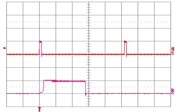
Fig. 3.3V.18: Load current (top trace, 20\ \text{A}/\text{div} ., 20\ \text{ms}/\text{div} .) into a 10\ \text{m}\Omega short circuit during restart, at V_{in} = 24\ \text{V} . Bottom trace ( 20\ \text{A}/\text{div} ., 1\ \text{ms}/\text{div} .) is an expansion of the on-time portion of the top trace.
