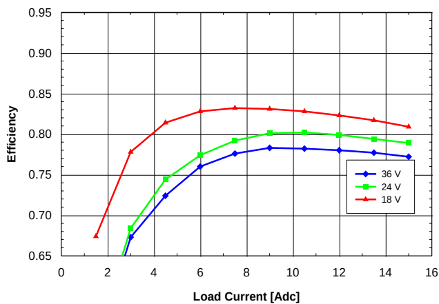
Fig. 1.0V.5: Efficiency vs. load current and input voltage for SQ24T/S15010 converter mounted vertically with air flowing from pin 3 to pin 1 at a rate of 300 LFM (1.5 m/s) and T_a = 25^{\circ}C .
