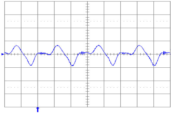
Fig. 1.5V.13: Output voltage ripple (20 mV/div.) at full rated load current into a resistive load with C_o = 10\ \mu\text{F} tantalum + 1\ \mu\text{F} ceramic and V_{in} = 24\ \text{V} . Time scale: 1\ \mu\text{s}/\text{div} .
