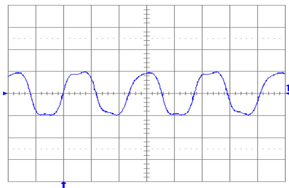
Fig. 5.0V.13: Output voltage ripple (20 mV/div.) at full rated load current into a resistive load with C_o = 10\ \mu\text{F} tantalum + 1\ \mu\text{F} ceramic and V_{in} = 24\ \text{V} . Time scale: 1\ \mu\text{s}/\text{div} .
