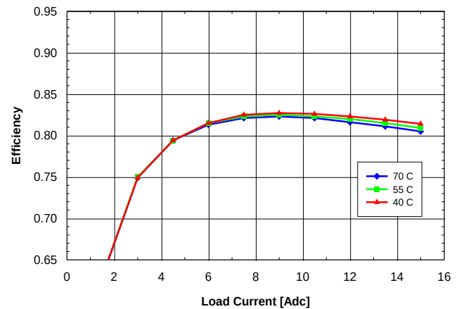
Fig. 1.2V.6: Efficiency vs. load current and ambient temperature for SQ24T/S15012 converter mounted vertically with V_{in} = 24V and air flowing from pin 3 to pin 1 at a rate of 200 LFM (1.0 m/s).
