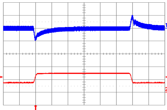
Fig. 1.2V.11: Output voltage response to load current step-change (3.75 A – 7.5 A – 3.75 A) at V_{in} = 24\text{V} . Top trace: output voltage (100 mV/div.). Bottom trace: load current (5 A/div.). Current slew rate: 0.1 A/ \mu\text{s} . C_o = 1\text{ }\mu\text{F} ceramic. Time scale: 0.2 ms/div.
