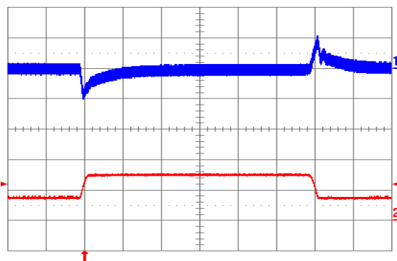
Fig. 2.0V.11: Output voltage response to load current step-change (3.75A – 7.5A – 3.75A) at V_{in} = 24\text{V} . Top trace: output voltage (100 mV/div.). Bottom trace: load current (5 A/div.). Current slew rate: 0.1 A/µs. C_o = 1\text{ }\mu\text{F} ceramic. Time scale: 0.2 ms/div.
