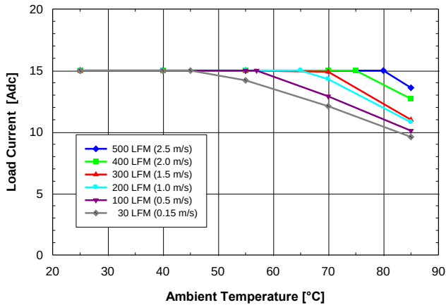
Fig. 3.3V.1: Available load current vs. ambient air temperature and airflow rates for SQ24T15033 converter with B height pins mounted vertically with V_{in} = 24V , air flowing from pin 3 to pin 1 and maximum FET temperature \leq 120^{\circ}C .
