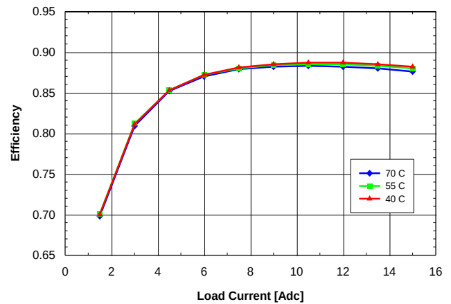
Fig. 3.3V.6: Efficiency vs. load current and ambient temperature for SQ24T/S15033 converter mounted vertically with V_{in} = 24V and air flowing from pin 3 to pin 1 at a rate of 200 LFM (1.0 m/s).
