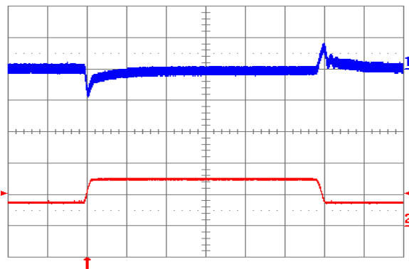
Fig. 1.8V.11: Output voltage response to load current step-change (3.75A – 7.5A – 3.75A) at V_{in} = 24\text{V} . Top trace: output voltage (100 mV/div.). Bottom trace: load current (5 A/div.). Current slew rate: 0.1 A/µs. C_o = 1\text{ }\mu\text{F} ceramic. Time scale: 0.2 ms/div.
