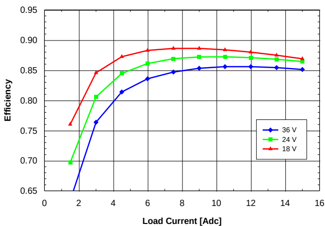
Fig. 2.5V.5: Efficiency vs. load current and input voltage for SQ24T/S15025 converter mounted vertically with air flowing from pin 3 to pin 1 at a rate of 300 LFM (1.5 m/s) and T_a = 25^{\circ}C .
