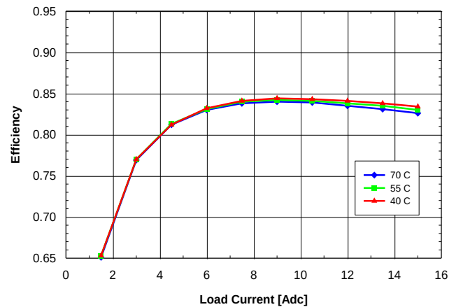
Fig. 1.5V.6: Efficiency vs. load current and ambient temperature for SQ24T/S15015 converter mounted vertically with V_{in} = 24V and air flowing from pin 3 to pin 1 at a rate of 200 LFM (1.0 m/s).
