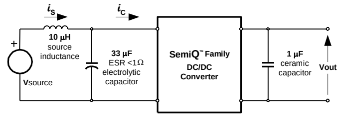
Fig. 1.5V.14: Test setup for measuring input reflected ripple currents, i_c and i_s .
