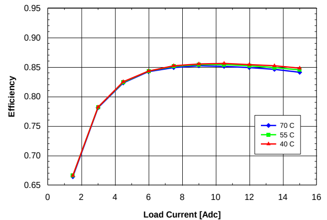
Fig. 1.8V.6: Efficiency vs. load current and ambient temperature for SQ24T/S15018 converter mounted vertically with V_{in} = 24V and air flowing from pin 3 to pin 1 at a rate of 200 LFM (1.0 m/s).
