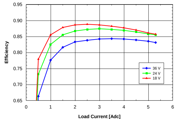
Fig. 8.0V.2: Efficiency vs. load current and input voltage for SQ24T/S05080 converter mounted vertically with air flowing from pin 3 to pin 1 at a rate of 300 LFM (1.5 m/s) and Ta = 25°C.
