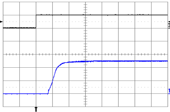
Fig. 5.0V.9: Turn-on transient at full rated load current (resistive) with no output capacitor at V_{in} = 24\text{V} , triggered via ON/OFF pin. Top trace: ON/OFF signal (5 V/div.). Bottom trace: output voltage (2 V/div.). Time scale: 2 ms/div.
