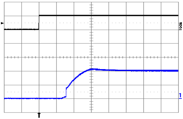
Fig. 1.0V.10: Turn-on transient at full rated load current (resistive) plus 10,000 µF at V_{in} = 24\text{V} , triggered via ON/OFF pin. Top trace: ON/OFF signal (5 V/div.). Bottom trace: output voltage (0.5 V/div.). Time scale: 1 ms/div.
