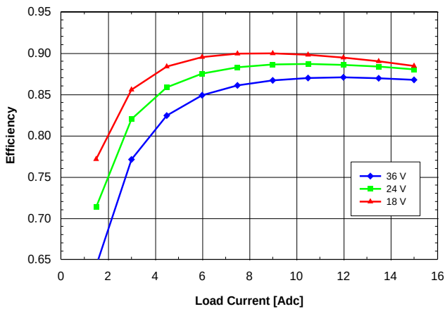
Fig. 3.3V.5: Efficiency vs. load current and input voltage for SQ24T/S15033 converter mounted vertically with air flowing from pin 3 to pin 1 at a rate of 300 LFM (1.5 m/s) and T_a = 25^{\circ}C .
