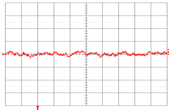
Fig. 5.0V.16: Input reflected ripple current, i_s (10 mA/div.), measured through 10\ \mu\text{H} at the source at full rated load current and V_{in} = 24\ \text{V} . Refer to Fig. 5.0V.14 for test setup. Time scale: 1\ \mu\text{s}/\text{div} .
