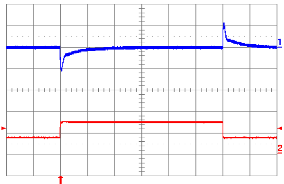
Fig. 1.0V.12: Output voltage response to load current step-change (3.75 A – 7.5 A – 3.75 A) at V_{in} = 24\text{V} . Top trace: output voltage (100 mV/div.). Bottom trace: load current (5 A/div.). Current slew rate: 5 A/µs. C_o = 450\text{ µF} tantalum + 1 µF ceramic. Time scale: 0.2 ms/div.
