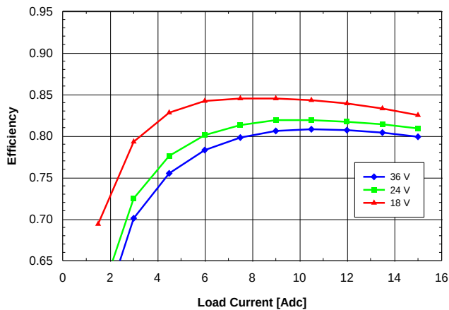
Fig. 1.2V.5: Efficiency vs. load current and input voltage for SQ24T/S15012 converter mounted vertically with air flowing from pin 3 to pin 1 at a rate of 300 LFM (1.5 m/s) and T_a = 25^{\circ}C .
