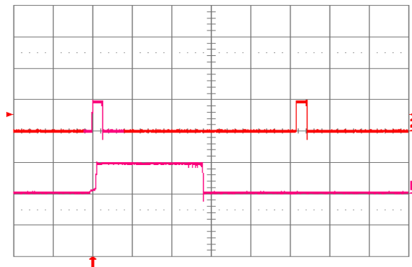
Fig. 1.5V.18: Load current (top trace, 20 A/div., 20 ms/div.) into a 10\ \text{m}\Omega short circuit during restart, at V_{in} = 24\ \text{V} . Bottom trace (20 A/div., 2 ms/div.) is an expansion of the on-time portion of the top trace.
