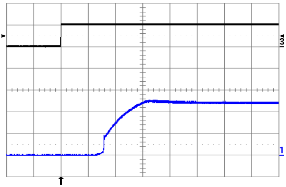
Fig. 1.2V.10: Turn-on transient at full rated load current (resistive) plus 10,000 \mu\text{F} at V_{in} = 24\text{V} , triggered via ON/OFF pin. Top trace: ON/OFF signal (5 V/div.). Bottom trace: output voltage (0.5 V/div.). Time scale: 1 ms/div.
