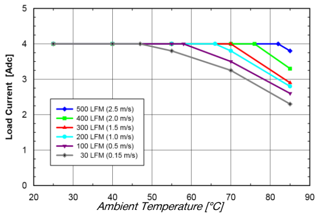
Fig. 12V.1: Available load current vs. ambient air temperature and airflow rates for SQ24T04120 converter with B height pins mounted vertically with V_{in} = 24V , air flowing from pin 3 to pin 1 and maximum FET temperature \leq 120^{\circ}C .
