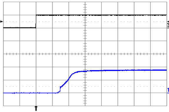
Fig. 1.8V.9: Turn-on transient at full rated load current (resistive) with no output capacitor at V_{in} = 24\text{V} , triggered via ON/OFF pin. Top trace: ON/OFF signal (5 V/div.). Bottom trace: output voltage (1 V/div.). Time scale: 1 ms/div.
