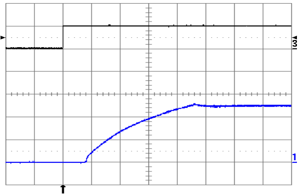
Fig. 5.0V.10: Turn-on transient at full rated load current (resistive) plus 10,000 µF at V_{in} = 24\text{V} , triggered via ON/OFF pin. Top trace: ON/OFF signal (5 V/div.). Bottom trace: output voltage (2 V/div.). Time scale: 2 ms/div.
