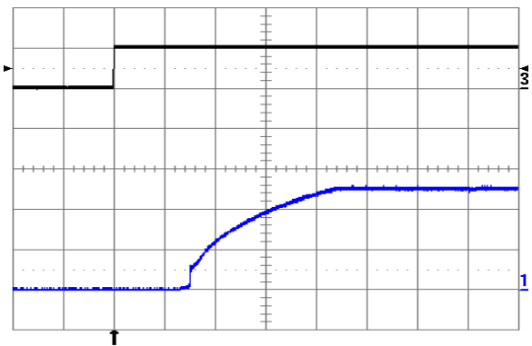
Fig. 2.5V.10: Turn-on transient at full rated load current (resistive) plus 10,000 \mu\text{F} at V_{in} = 24\text{V} , triggered via ON/OFF pin. Top trace: ON/OFF signal (5 V/div.). Bottom trace: output voltage (1 V/div.). Time scale: 1 ms/div.
