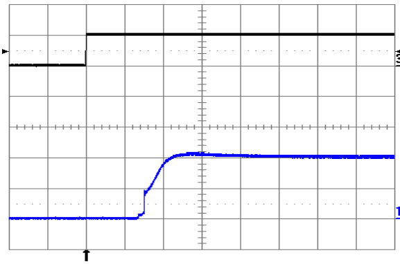
Fig. 1.0V.9: Turn-on transient at full rated load current (resistive) with no output capacitor at V_{in} = 24\text{V} , triggered via ON/OFF pin. Top trace: ON/OFF signal (5 V/div.). Bottom trace: output voltage (0.5 V/div.). Time scale: 1 ms/div.
