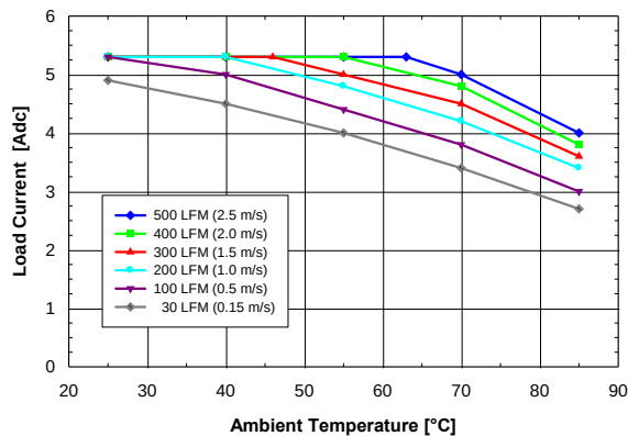
Fig. 8.0V.1: Available load current vs. ambient air temperature and airflow rates for SQ24T05080 converter with D height pins mounted vertically with Vin = 24 V, air flowing from pin 3 to pin 1 and maximum FET temperature ≤ 120°C.
