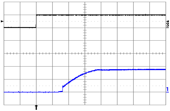
Fig. 1.8V.10: Turn-on transient at full rated load current (resistive) plus 10,000 µF at V_{in} = 24\text{V} , triggered via ON/OFF pin. Top trace: ON/OFF signal (5 V/div.). Bottom trace: output voltage (1 V/div.). Time scale: 1 ms/div.
