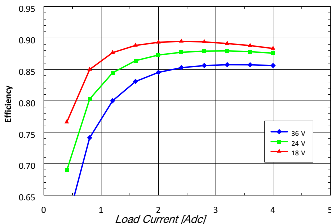
Fig. 12V.5: Efficiency vs. load current and input voltage for SQ24T/S04120 converter mounted vertically with air flowing from pin 3 to pin 1 at a rate of 300 LFM (1.5 m/s) and T_a = 25^{\circ}C .
