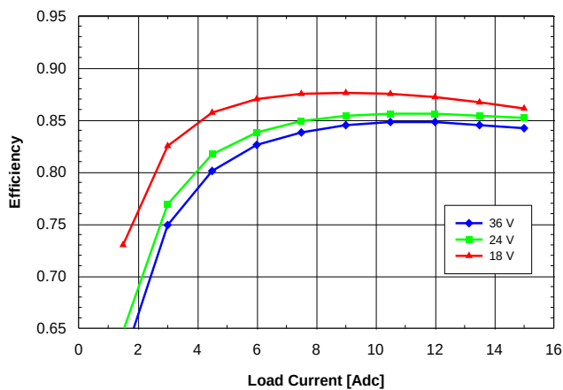
Fig. 2.0V.5: Efficiency vs. load current and input voltage for SQ24T/S15020 converter mounted vertically with air flowing from pin 3 to pin 1 at a rate of 300 LFM (1.5 m/s) and T_a = 25^{\circ}C .
