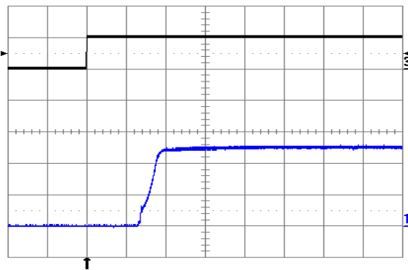
Fig. 2.5V.9: Turn-on transient at full rated load current (resistive) with no output capacitor at V_{in} = 24\text{V} , triggered via ON/OFF pin. Top trace: ON/OFF signal (5 V/div.). Bottom trace: output voltage (1 V/div.). Time scale: 1 ms/div.
