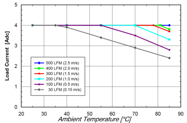
Fig. 12V.2: Available load current vs. ambient air temperature and airflow rates for SQ24T04120 converter mounted horizontally with B height pins with V_{in} = 24V , air flowing from pin 3 to pin 1 and maximum FET temperature \leq 120^{\circ}C .
