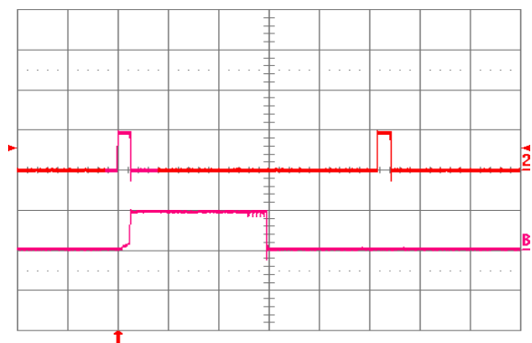
Fig. 1.2V.18: Load current (top trace, 20 A/div., 20 ms/div.) into a 10\ \text{m}\Omega short circuit during restart, at V_{in} = 24\ \text{V} . Bottom trace (20 A/div., 2 ms/div.) is an expansion of the on-time portion of the top trace.
