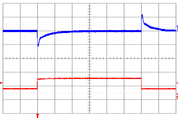
Fig. 1.5V.12: Output voltage response to load current step-change (3.75 A – 7.5 A – 3.75 A) at V_{in} = 24\text{V} . Top trace: output voltage (100 mV/div.). Bottom trace: load current (5 A/div.). Current slew rate: 5 A/ \mu\text{s} . C_o = 450\text{ }\mu\text{F} tantalum + 1 \mu\text{F} ceramic. Time scale: 0.2 ms/div.
