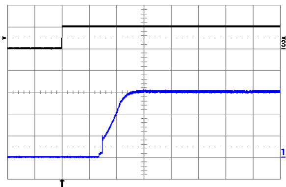
Fig. 1.5V.9: Turn-on transient at full rated load current (resistive) with no output capacitor at V_{in} = 24\text{V} , triggered via ON/OFF pin. Top trace: ON/OFF signal (5 V/div.). Bottom trace: output voltage (0.5 V/div.). Time scale: 1 ms/div.
