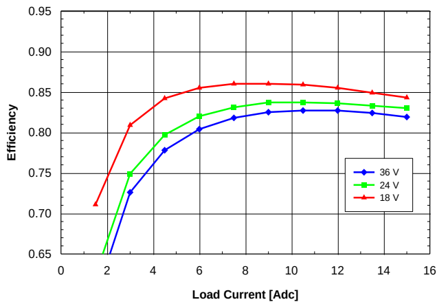
Fig. 1.5V.5: Efficiency vs. load current and input voltage for SQ24T/S15015 converter mounted vertically with air flowing from pin 3 to pin 1 at a rate of 300 LFM (1.5 m/s) and T_a = 25^{\circ}C .
