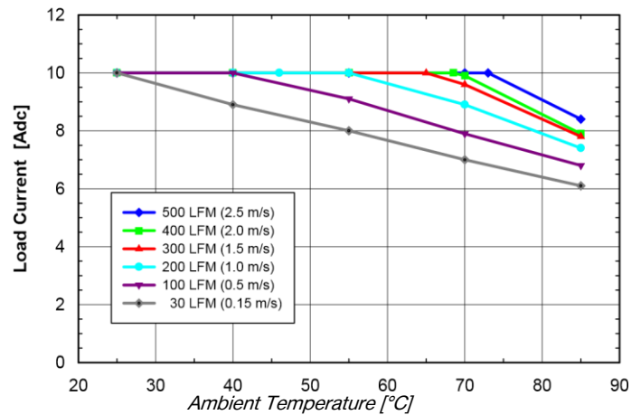
Fig. 5.0V.2: Available load current vs. ambient air temperature and airflow rates for SQ24T10050 converter with B height pins mounted horizontally with V_{in} = 24V , air flowing from pin 3 to pin 1 and maximum FET temperature \leq 120^{\circ}C .
