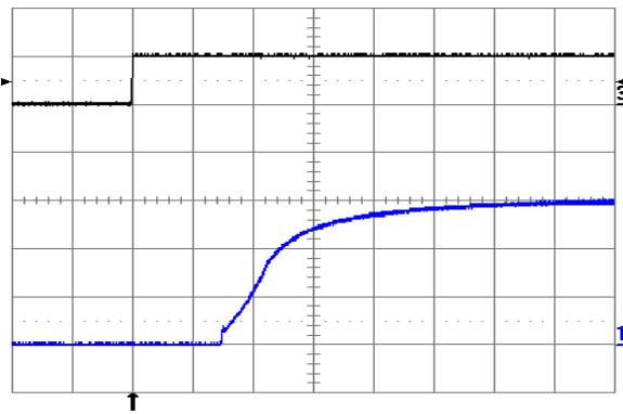
Fig. 6.0V.9: Turn-on transient at full rated load current (resistive) with no output capacitor at V_{in} = 24\text{V} , triggered via ON/OFF pin. Top trace: ON/OFF signal (5 V/div.). Bottom trace: output voltage (2 V/div.). Time scale: 1 ms/div.
