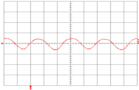
Fig. 2.0V.15: Input reflected ripple current, i_c (100 mA/div.), measured at input terminals at full rated load current and V_{in} = 24\ \text{V} . Refer to Fig. 2.0V.14 for test setup. Time scale: 1\ \mu\text{s}/\text{div} .
