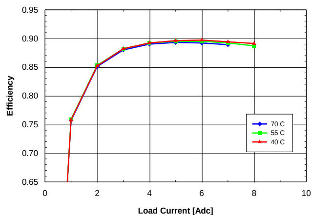
Fig. 6.0V.6: Efficiency vs. load current and ambient temperature for SQ24T/S08060 converter mounted vertically with V_{in} = 24V and air flowing from pin 3 to pin 1 at a rate of 200 LFM (1.0 m/s).
