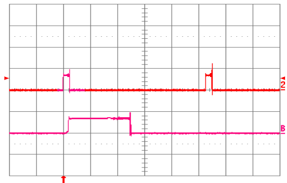
Fig. 6.0V.18: Load current (top trace, 20 A/div., 20 ms/div.) into a 10\ \text{m}\Omega short circuit during restart, at V_{in} = 24\ \text{V} . Bottom trace (20 A/div., 2 ms/div.) is an expansion of the on-time portion of the top trace.
