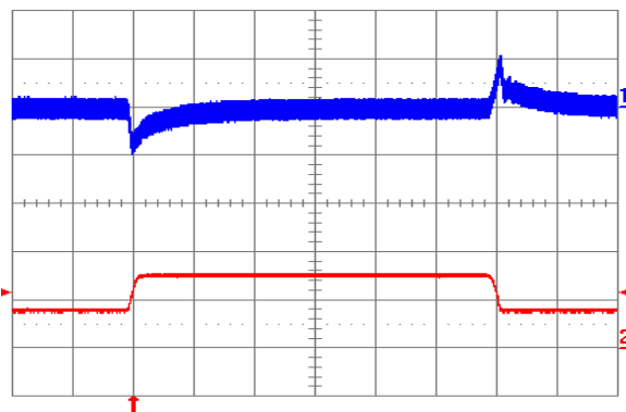
Fig. 2.5V.11: Output voltage response to load current step-change (3.75 A – 7.5 A – 3.75 A) at V_{in} = 24\text{V} . Top trace: output voltage (100 mV/div.). Bottom trace: load current (5 A/div.). Current slew rate: 0.1 A/ \mu\text{s} . C_o = 1 \mu\text{F} ceramic. Time scale: 0.2 ms/div.
