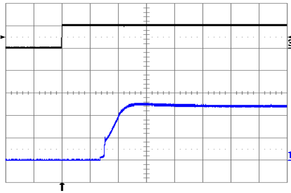
Fig. 1.2V.9: Turn-on transient at full rated load current (resistive) with no output capacitor at V_{in} = 24\text{V} , triggered via ON/OFF pin. Top trace: ON/OFF signal (5 V/div.). Bottom trace: output voltage (0.5 V/div.). Time scale: 1 ms/div.
