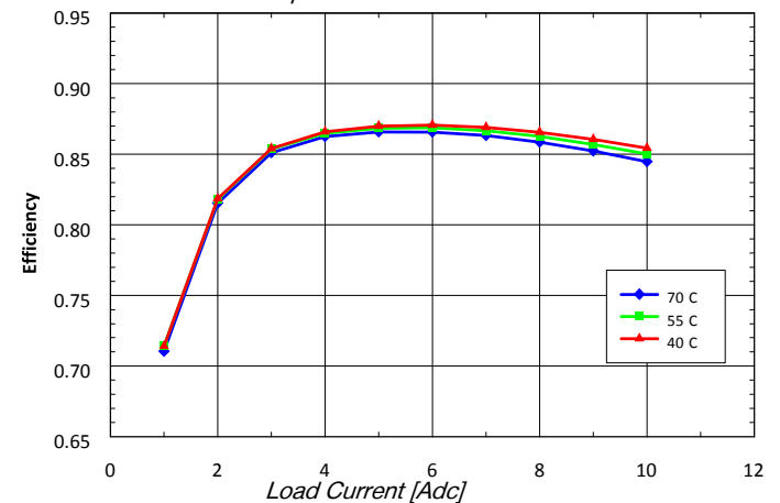
Fig. 5.0V.6: Efficiency vs. load current and ambient temperature for SQ24T/S10050 converter mounted vertically with V_{in} = 24V and air flowing from pin 3 to pin 1 at a rate of 200 LFM (1.0 m/s).
