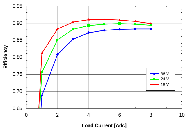
Fig. 6.0V.5: Efficiency vs. load current and input voltage for SQ24T/S08060 converter mounted vertically with air flowing from pin 3 to pin 1 at a rate of 300 LFM (1.5 m/s) and T_a = 25^{\circ}C .
