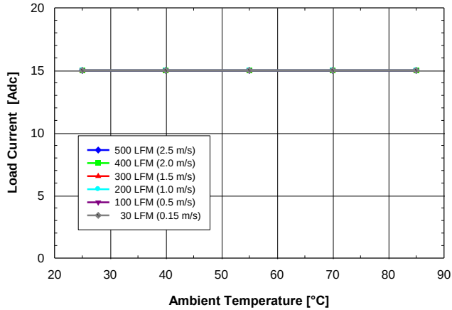
Fig. 1.5V.1: Available load current vs. ambient air temperature and airflow rates for SQ24T15015 converter with B height pins mounted vertically with V_{in} = 24V , air flowing from pin 3 to pin 1 and maximum FET temperature \leq 120^{\circ}C .
