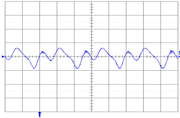
Fig. 1.2V.13: Output voltage ripple (20 mV/div.) at full rated load current into a resistive load with C_o = 10\ \mu\text{F} tantalum + 1\ \mu\text{F} ceramic and V_{in} = 24\ \text{V} . Time scale: 1\ \mu\text{s}/\text{div} .
