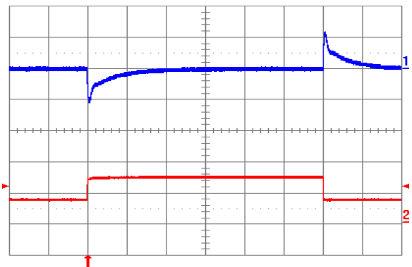
Fig. 1.2V.12: Output voltage response to load current step-change (3.75 A – 7.5 A – 3.75 A) at V_{in} = 24\text{V} . Top trace: output voltage (100 mV/div.). Bottom trace: load current (5 A/div.). Current slew rate: 5 A/ \mu\text{s} . C_o = 450\text{ }\mu\text{F} tantalum + 1 \mu\text{F} ceramic. Time scale: 0.2 ms/div.
