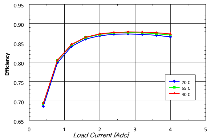
Fig. 12V.6: Efficiency vs. load current and ambient temperature for SQ24T/S04120 converter mounted vertically with V_{in} = 24V and air flowing from pin 3 to pin 1 at a rate of 200 LFM (1.0 m/s).
