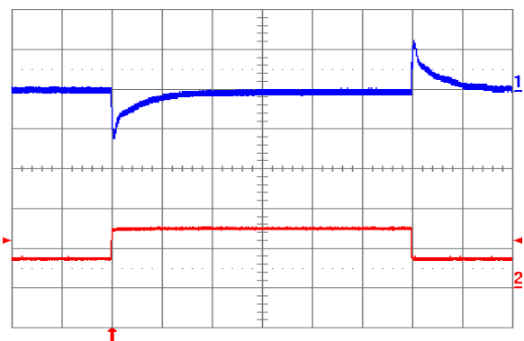
Fig. 2.0V.12: Output voltage response to load current step-change (3.75A – 7.5A – 3.75A) at V_{in} = 24\text{V} . Top trace: output voltage (100 mV/div.). Bottom trace: load current (5 A/div.). Current slew rate: 5 A/µs. C_o = 450\text{ }\mu\text{F} tantalum + 1 µF ceramic. Time scale: 0.2 ms/div.
