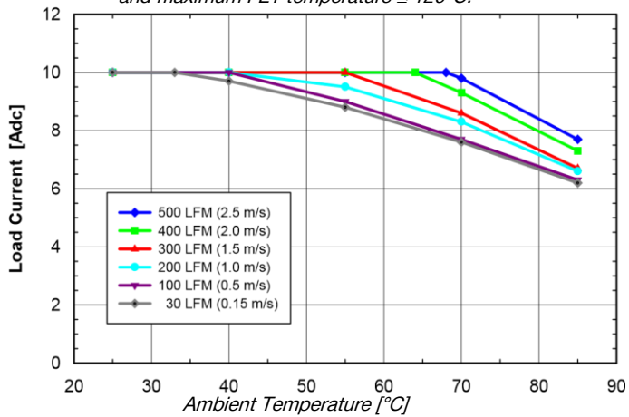
Fig. 5.0V.3: Available load current vs. ambient temperature and airflow rates for SQ24S10050 converter mounted vertically with V_{in} = 24V , air flowing from pin 3 to pin 1 and maximum FET temperature \leq 120^{\circ}C .
