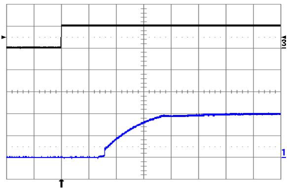
Fig. 2.0V.10: Turn-on transient at full rated load current (resistive) plus 10,000 µF at V_{in} = 24\text{V} , triggered via ON/OFF pin. Top trace: ON/OFF signal (5 V/div.). Bottom trace: output voltage (1 V/div.). Time scale: 1 ms/div.
