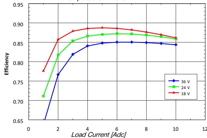
Fig. 5.0V.5: Efficiency vs. load current and input voltage for SQ24T/S10050 converter mounted vertically with air flowing from pin 3 to pin 1 at a rate of 300 LFM (1.5 m/s) and T_a = 25^{\circ}C .
