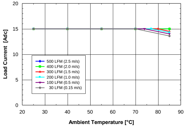
Fig. 1.8V.3: Available load current vs. ambient temperature and airflow rates for SQ24S15018 converter mounted vertically with V_{in} = 24V , air flowing from pin 3 to pin 1 and maximum FET temperature \leq 120^{\circ}C .
