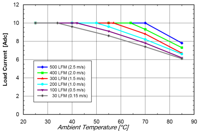
Fig. 5.0V.1: Available load current vs. ambient air temperature and airflow rates for SQ24T10050 converter with B height pins mounted vertically with V_{in} = 24V , air flowing from pin 3 to pin 1 and maximum FET temperature \leq 120^{\circ}C .
