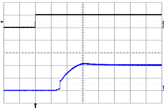
Fig. 1.0V.11: Turn-on transient at full rated load current (resistive) plus 10,000 µF at V_{in} = 24\text{V} , triggered via ON/OFF pin. Top trace: ON/OFF signal (5 V/div.). Bottom trace: output voltage (0.5 V/div.). Time scale: 1 ms/div.
